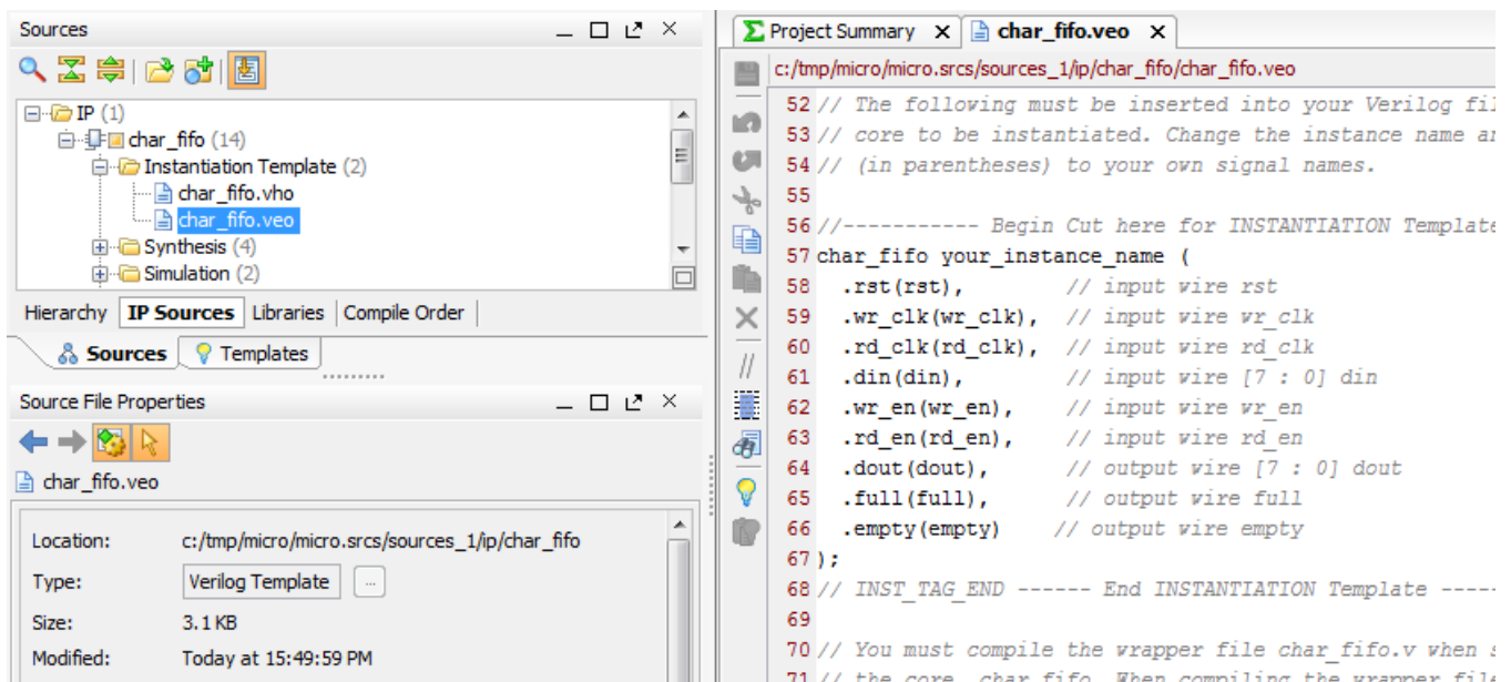
Figure 2-31: Instantiation Template
