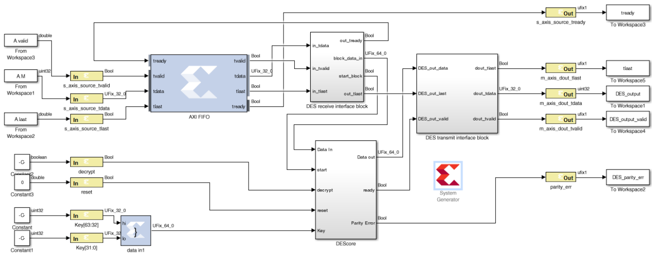
Figure 100: Lab9_1 Design
