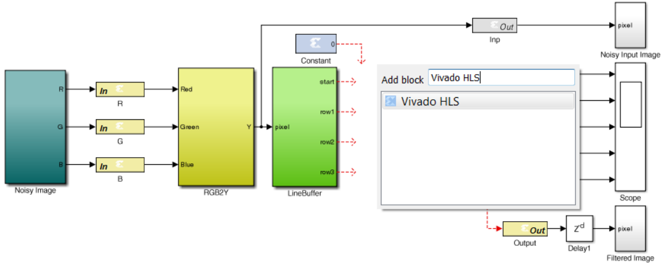
Figure 82: Adding a Vivado HLS Block
