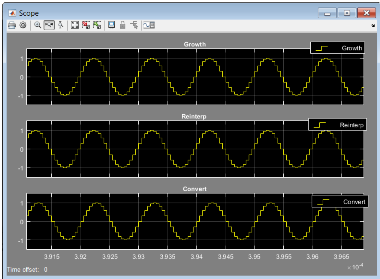
Figure 41: Updated Lab2_2 Design Scope
