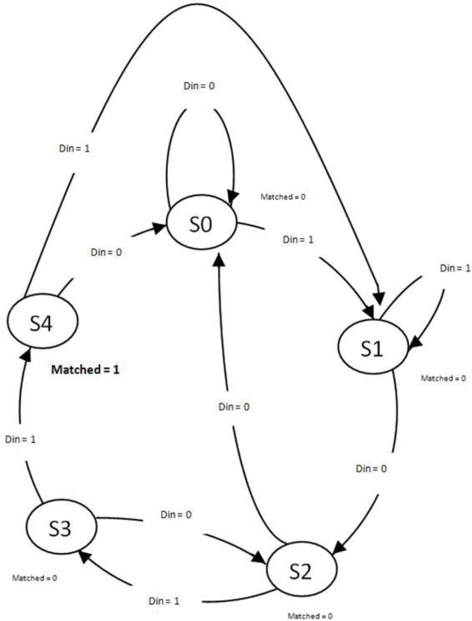
Figure 68: State Machine
