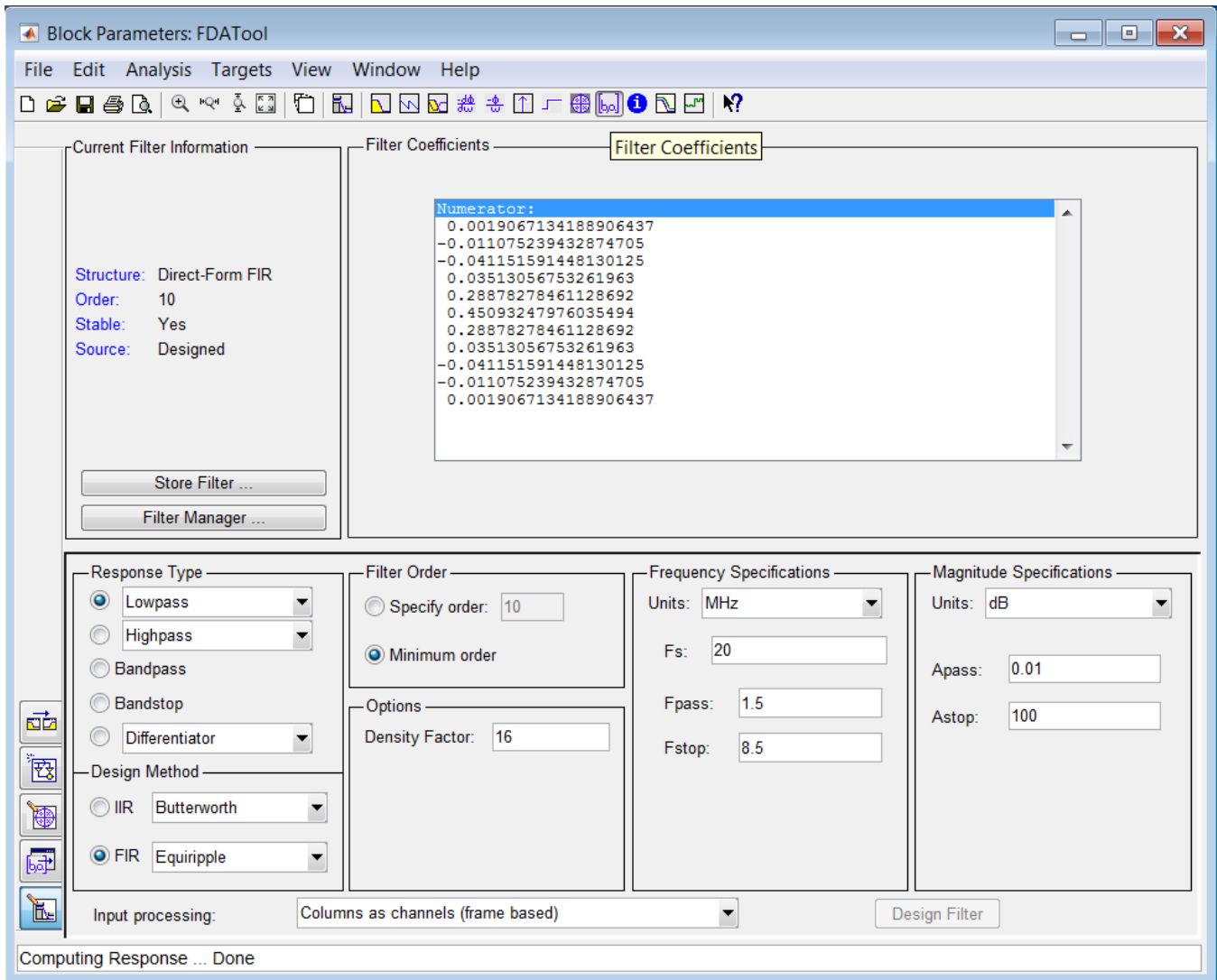
Figure 20: Lab1_2 Filter Coefficients
