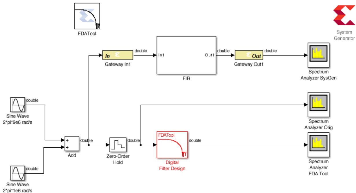
Figure 33: Initial Lab2_1 Design
