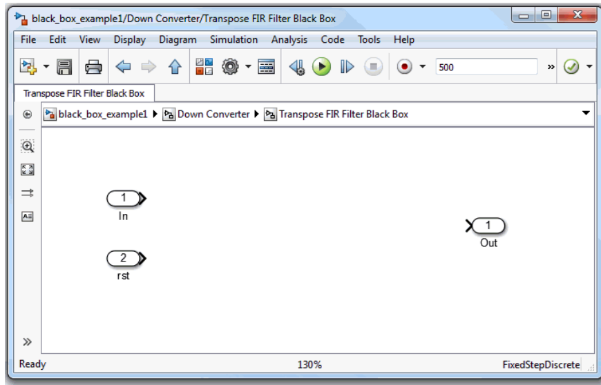
Figure 70: Lab6_1 Design: Transpose FIR Filter Black Box
