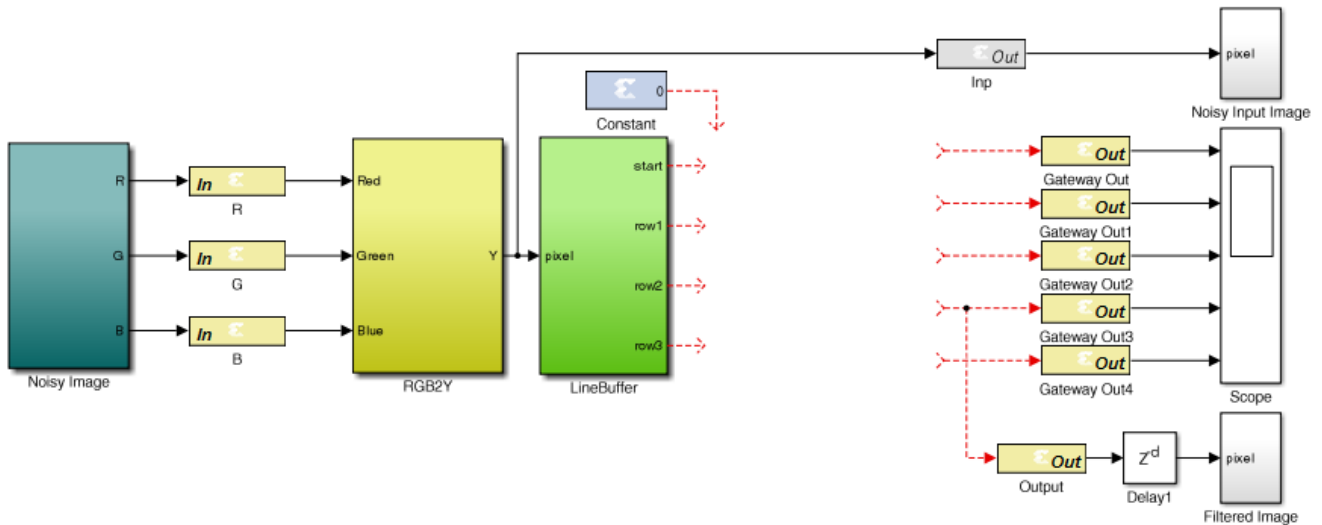
Figure 81: Lab7_1 Design
