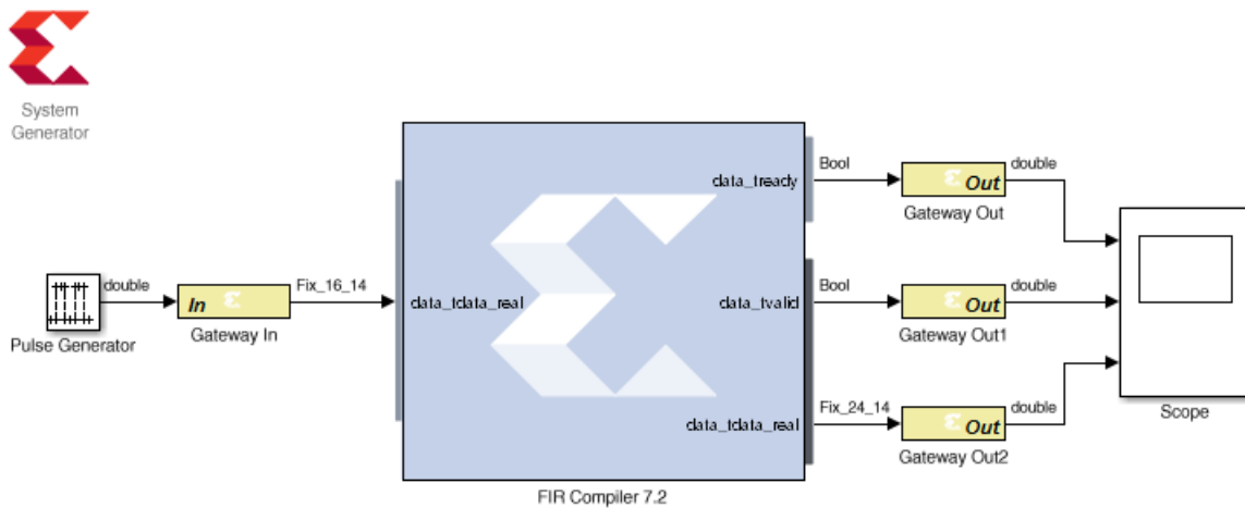
Figure 59: Initial Lab4_1 Design
