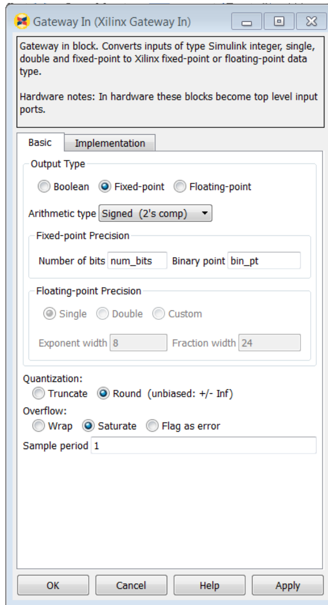
Figure 62: Lab4 Gateway In Properties
