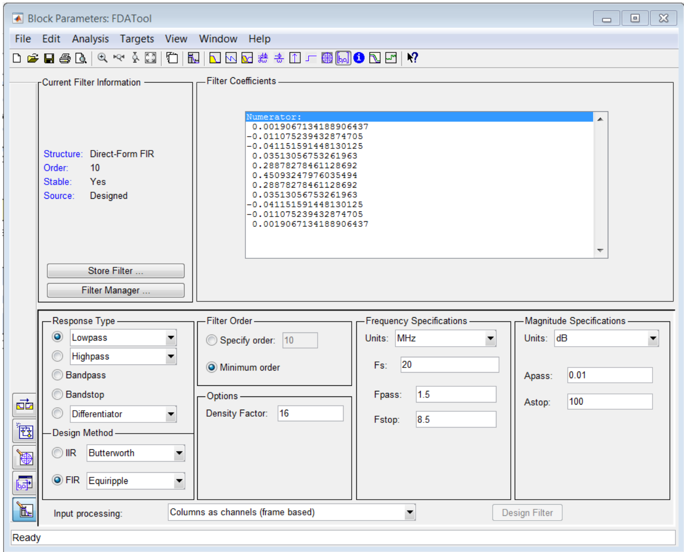
Figure 26: Lab1_3 Filter Specifications
