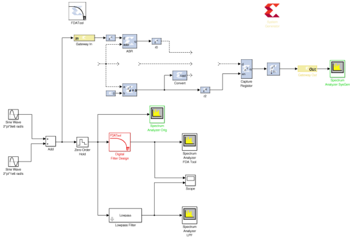
Figure 23: Initial Lab1_3 Design
