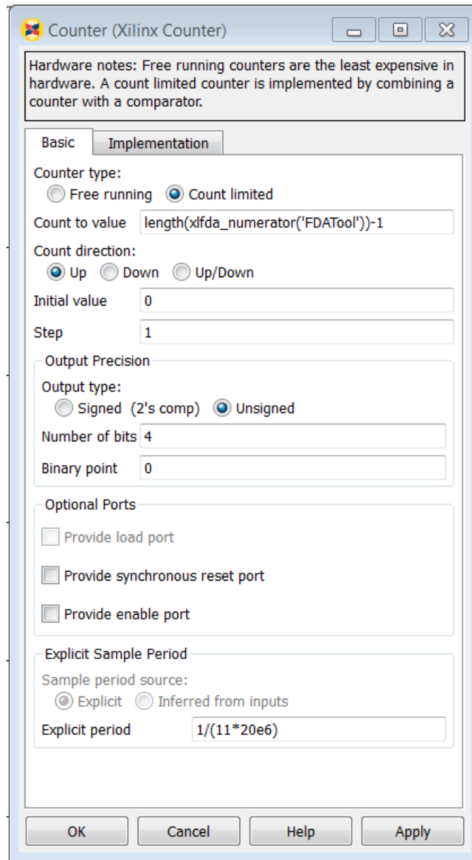
Figure 27: Counter Properties Editor
