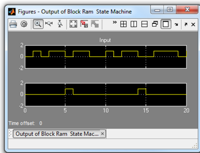
Figure 69: Lab5 Waveforms
