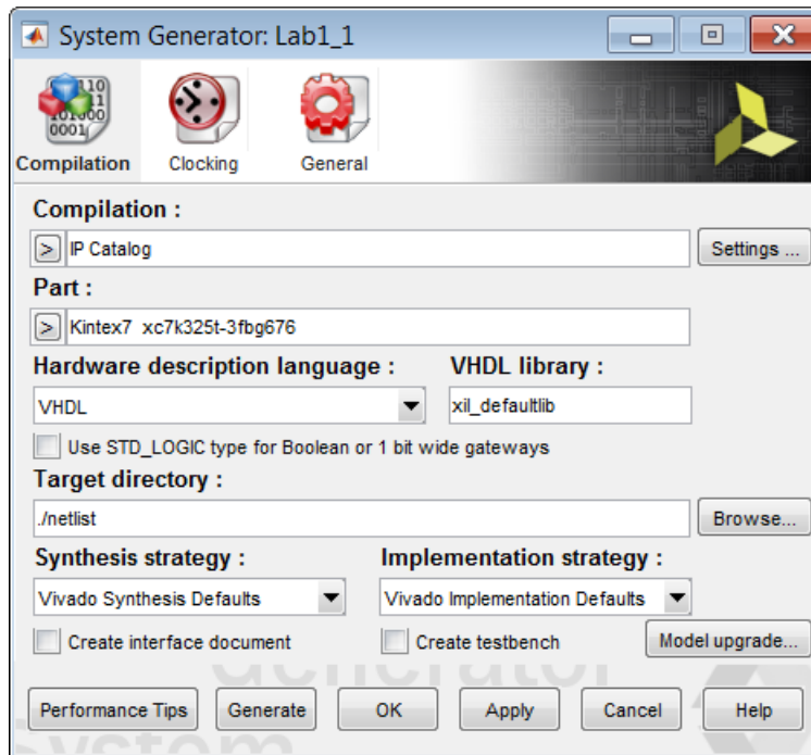
Figure 14: System Generator Token for Lab 1 Step 1
