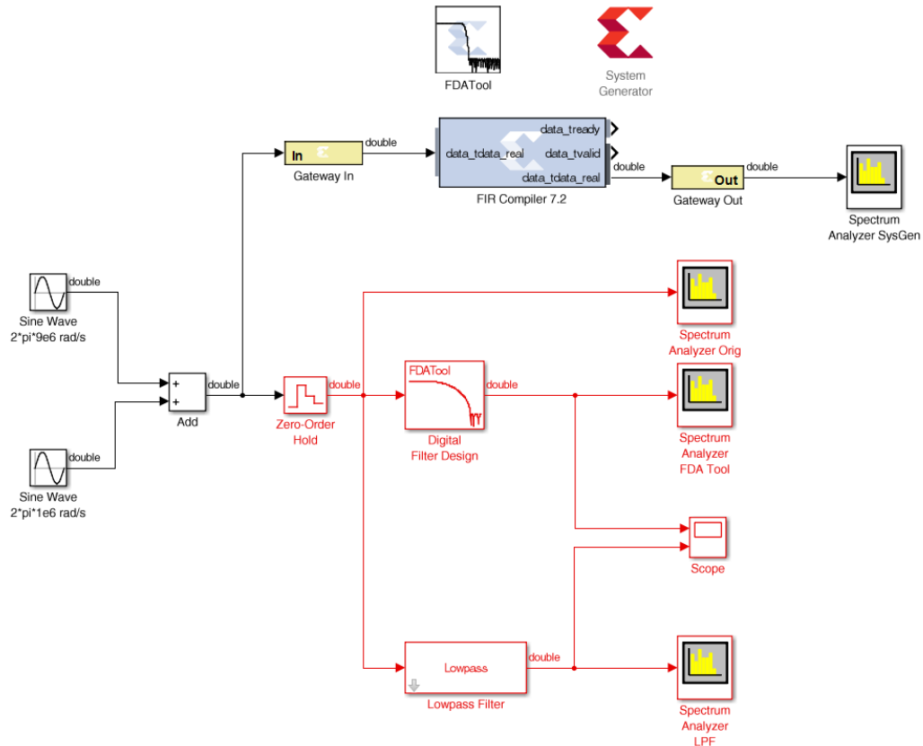
Figure 8: Initial System Generator Design
