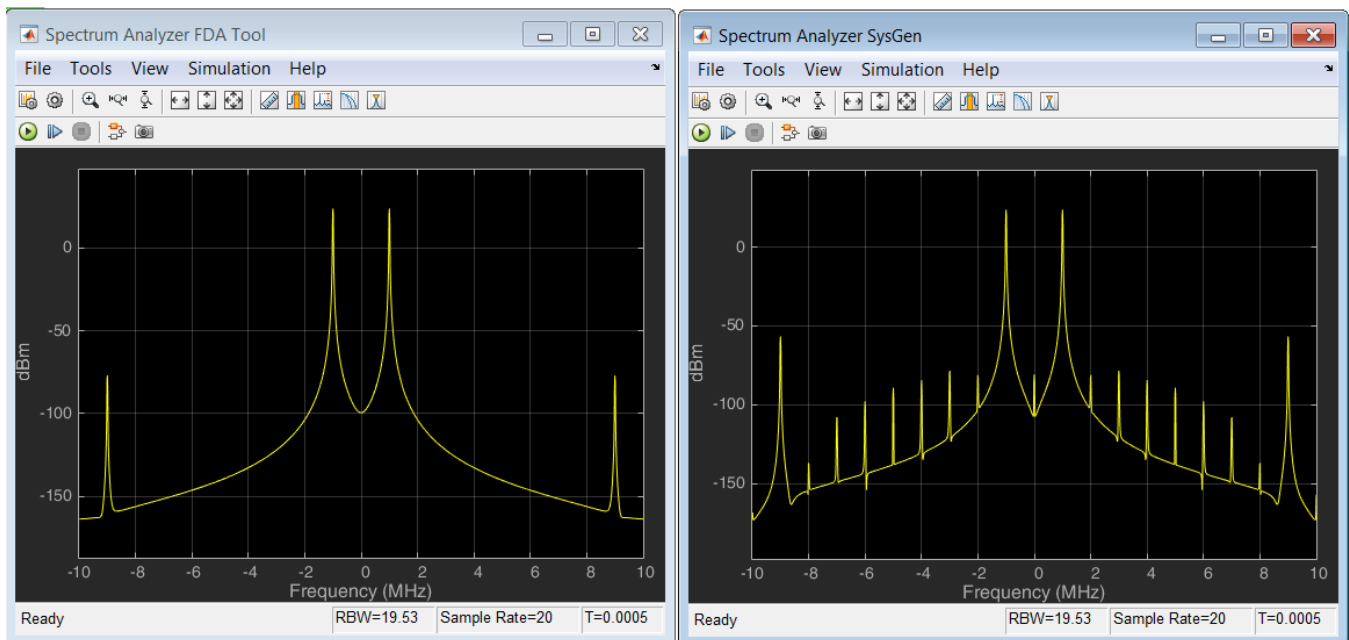
Figure 31: Discrete FIR Compiler Results
