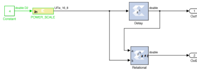
Figure 51: Modified CTRL Subsystem
