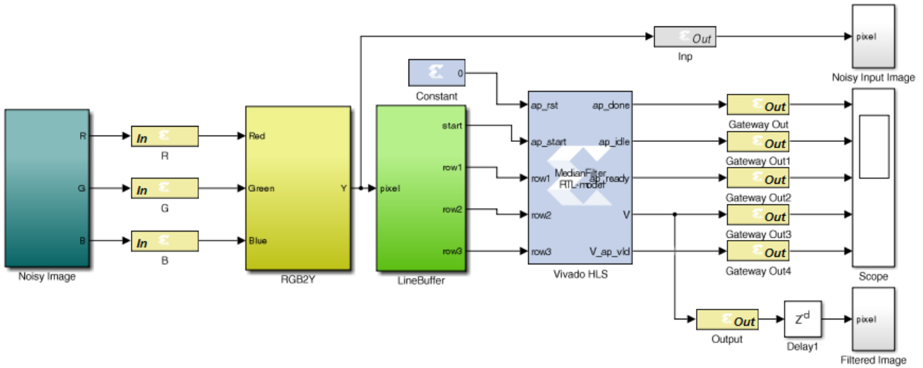
Figure 84: Completed Lab7_1 Design
