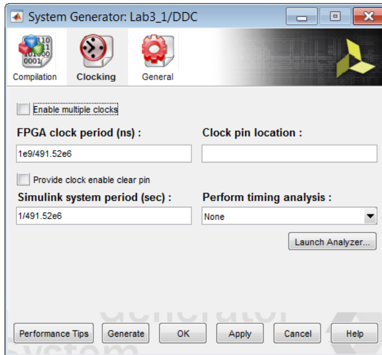
Figure 58: DDC Clock Domain
