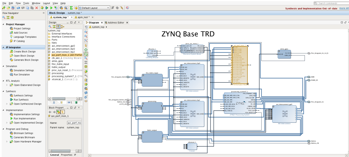
Figure 11-1: Zynq-7000 AP SoC Base TRD Hardware Block Diagram
