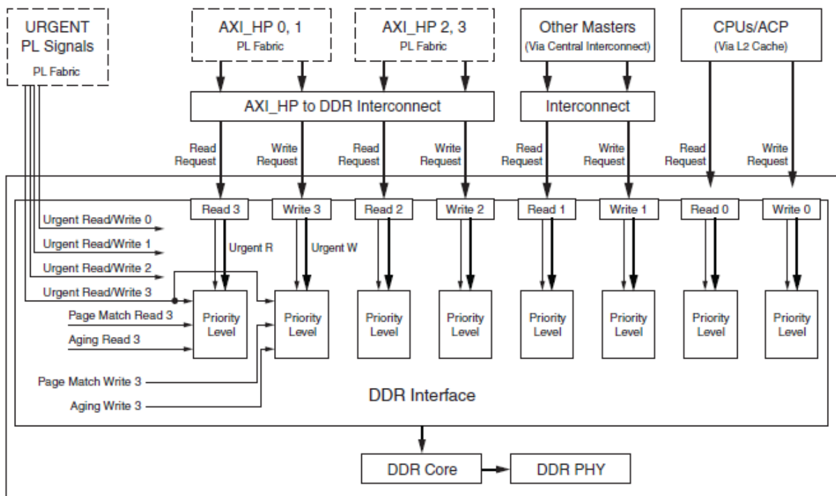
Figure 8-1: Block Diagram of Zynq-7000 AP SoC DDR Controller
