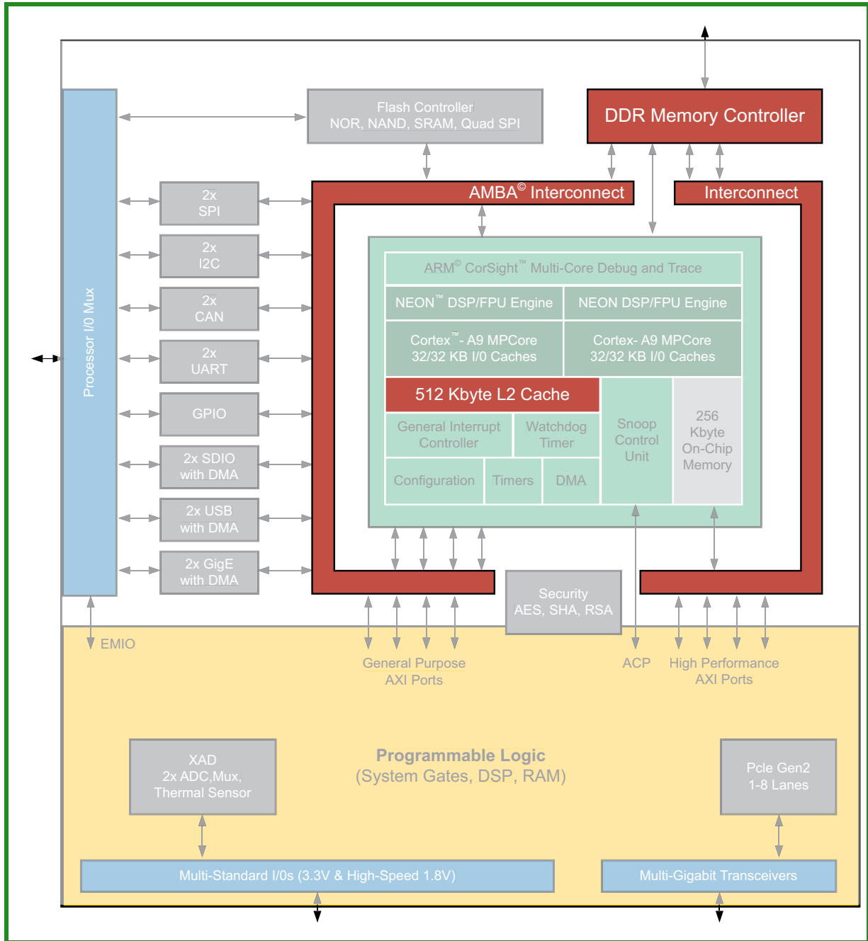
Figure 2-2: Zynq-7000 AP SoC Block Diagram with Shared Resources Highlighted
