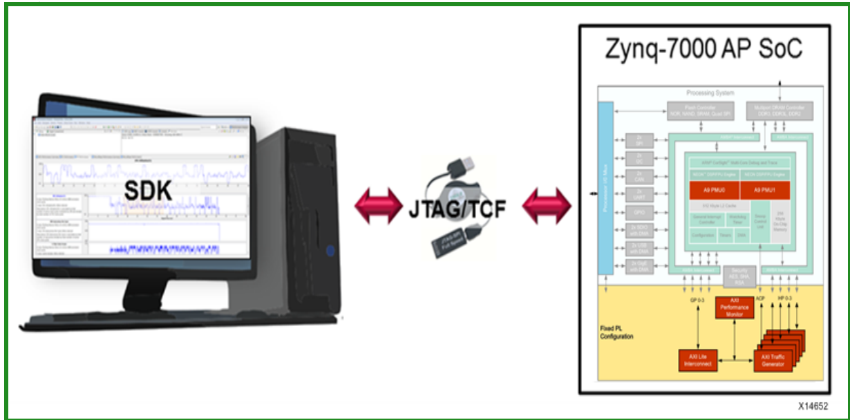
Figure 4-2: Host-Target Communication Infrastructure for SDK
