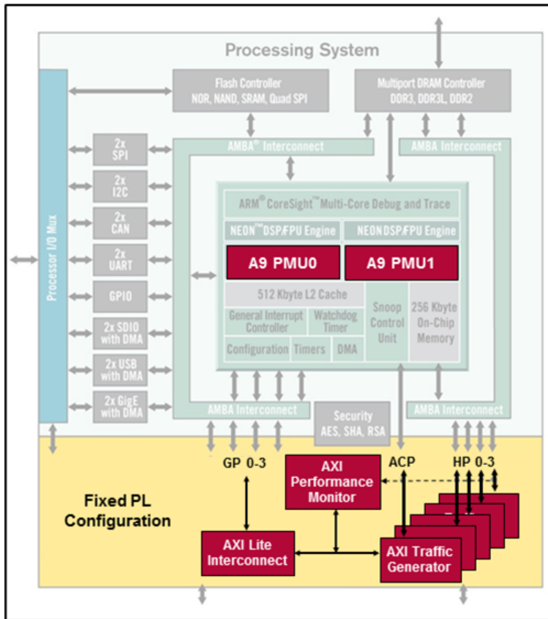
Figure 3-2: Pre-Defined SPM Design in Zynq-7000 AP SoC
