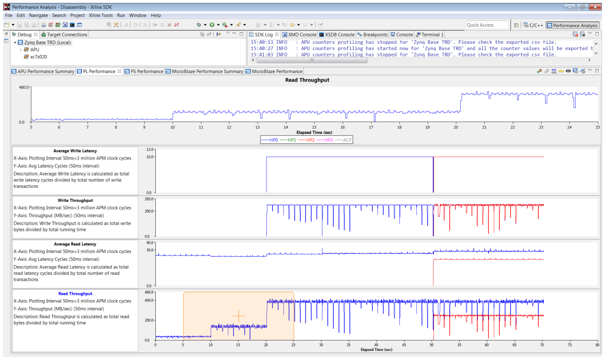
Figure 11-10: PL Performance Graphs of Zynq-7000 AP SoC Base TRD
