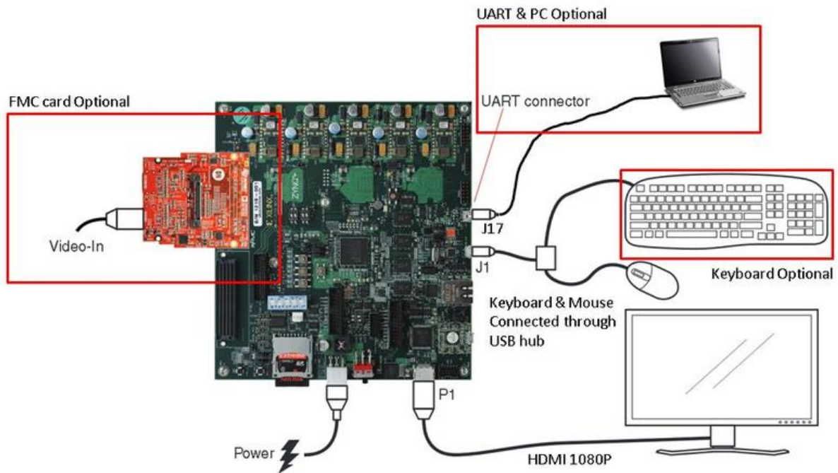
Figure 11-6: Connection Diagram of Zynq-7000 AP SoC Base TRD Using the ZC702 Board
