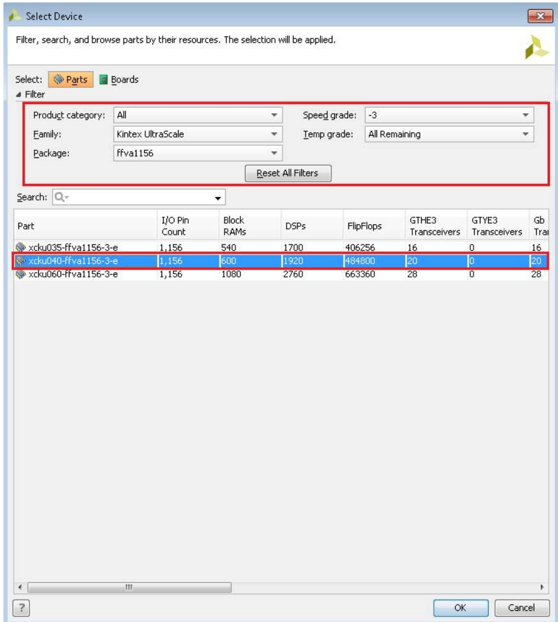
Figure 2-2: Select Device
