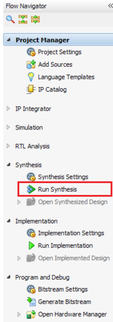
Figure 2-10: Run Synthesis
