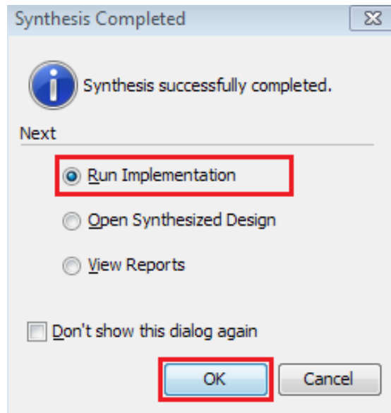
Figure 2-11: Synthesis Completed
