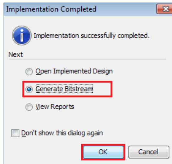
Figure 2-12: Implementation Completed
