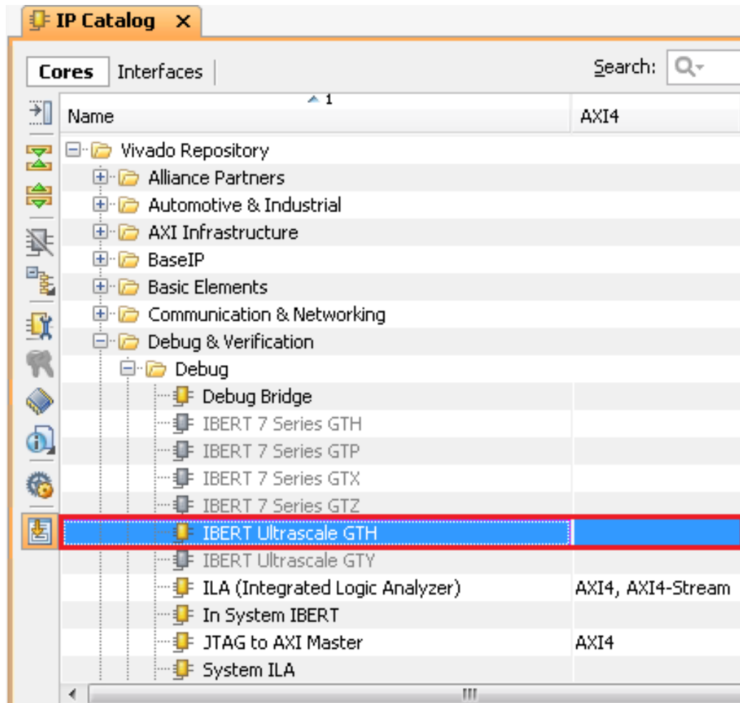
Figure 2-4: IP Catalog
