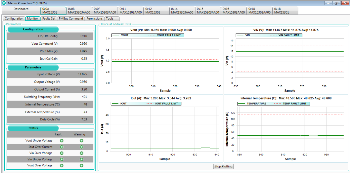
Figure 68: Monitoring a Rail - Voltage and Current
