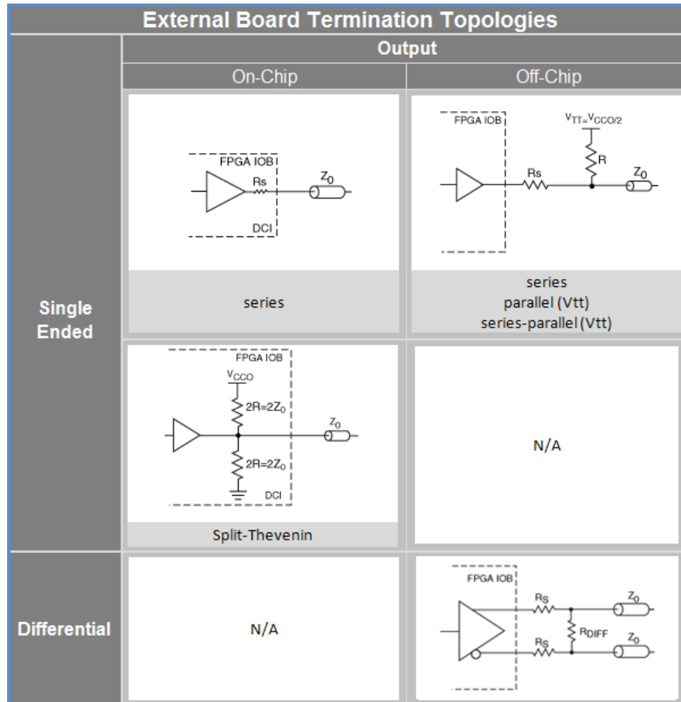
Figure 3-6: External I/O Termination Topologies (Virtex-6 and 7 Series Devices)
