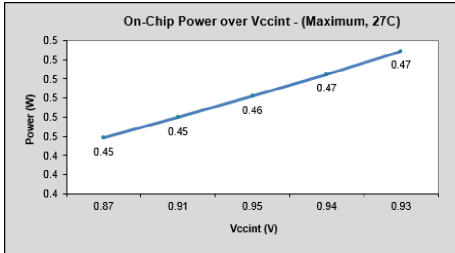
Figure 6-3: Graph displaying On-Chip Power Over Vccint
