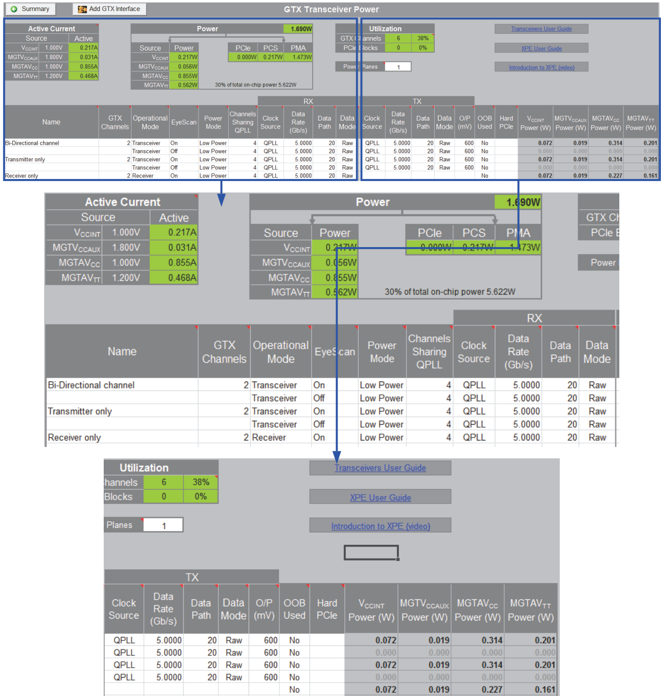
Figure 3-9: GT Power Sheet (Kintex-7 Devices) Illustrating Data Rate and Power Estimates
