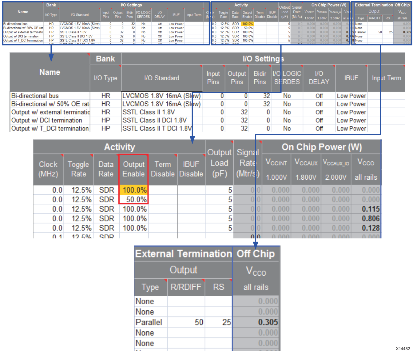
Figure 3-5: I/O Sheet - Effect of Output Enable Rate on Power Estimates for Inputs, Outputs, and Bidirectional I/Os (7 Series Devices)
