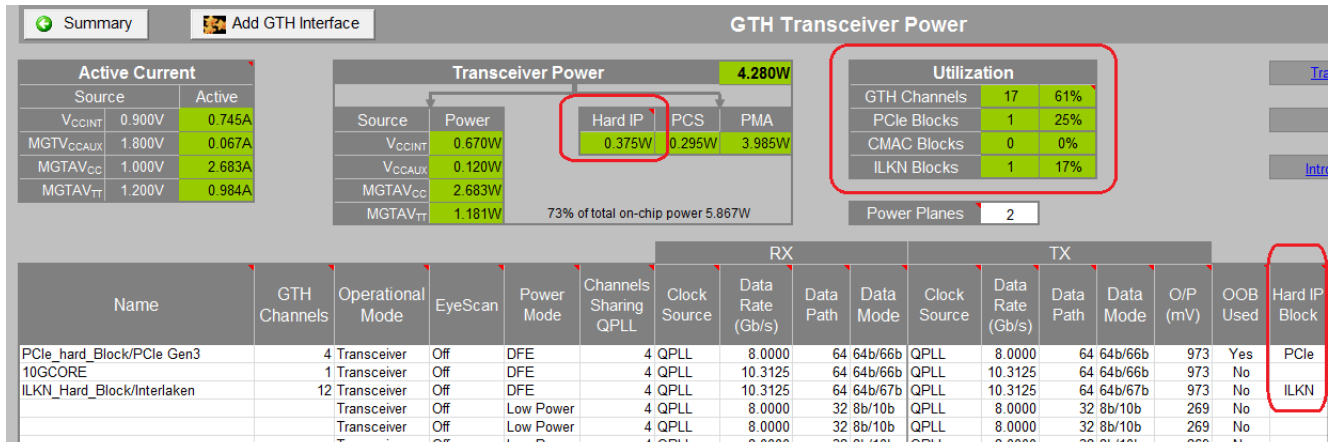
Figure 3-10: Hard IP Settings for UltraScale Devices
