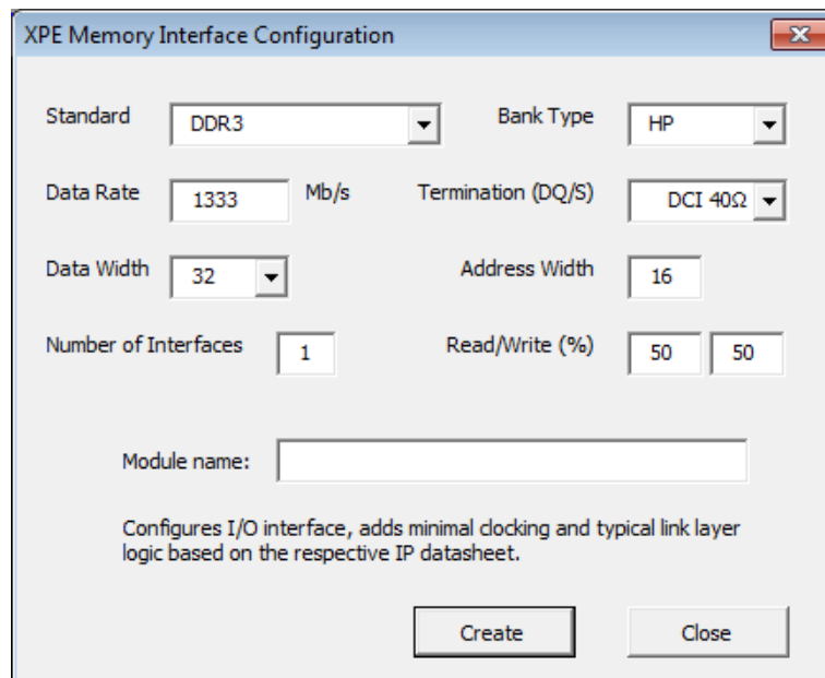
Figure 1-12: XPE Memory Interface Configuration Dialog Box (Virtex-7 Devices)
