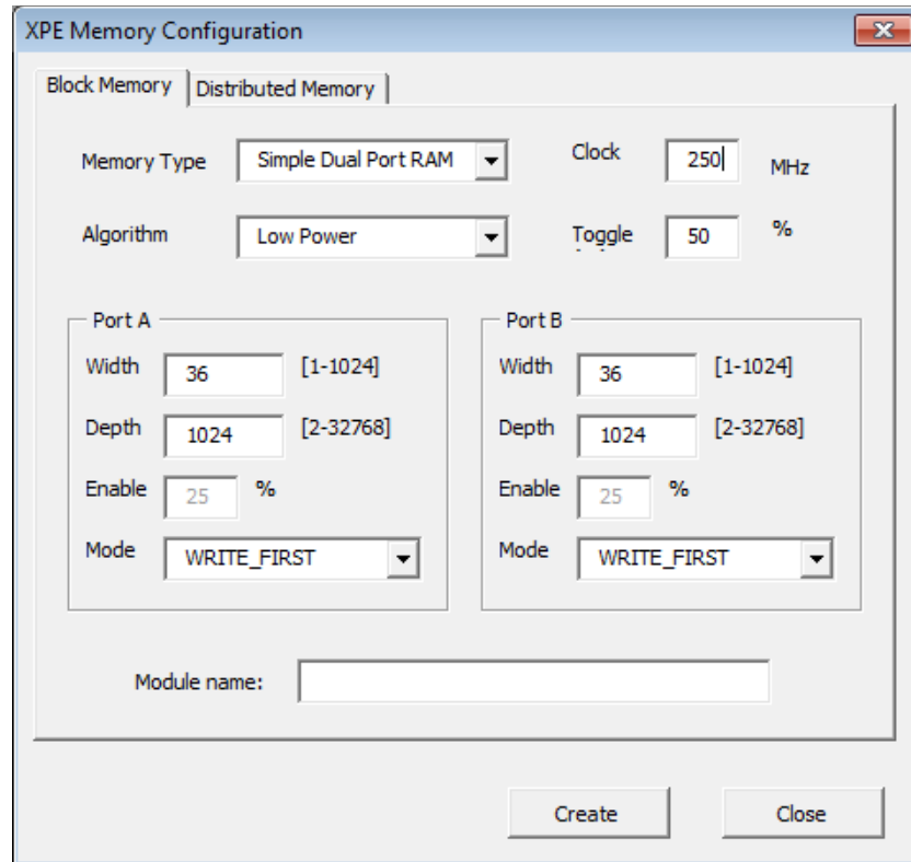
Figure 1-11: Block Memory Tab - XPE Memory Generator Dialog Box (Virtex-7 Devices)
