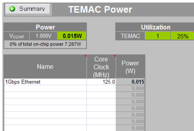
Figure 3-11: TEMAC Power Sheet (Virtex-6 Devices)
