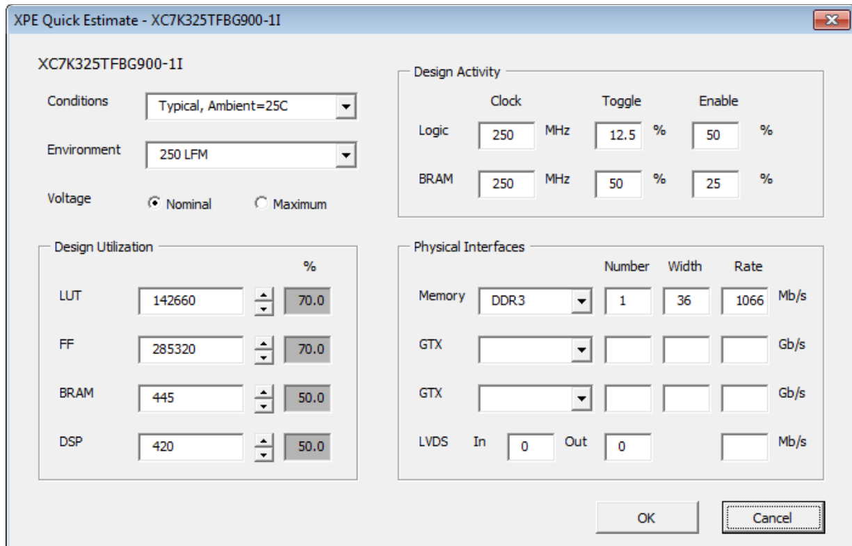
Figure 1-9: XPE Quick Estimate Dialog Box (Virtex-7 Devices)
