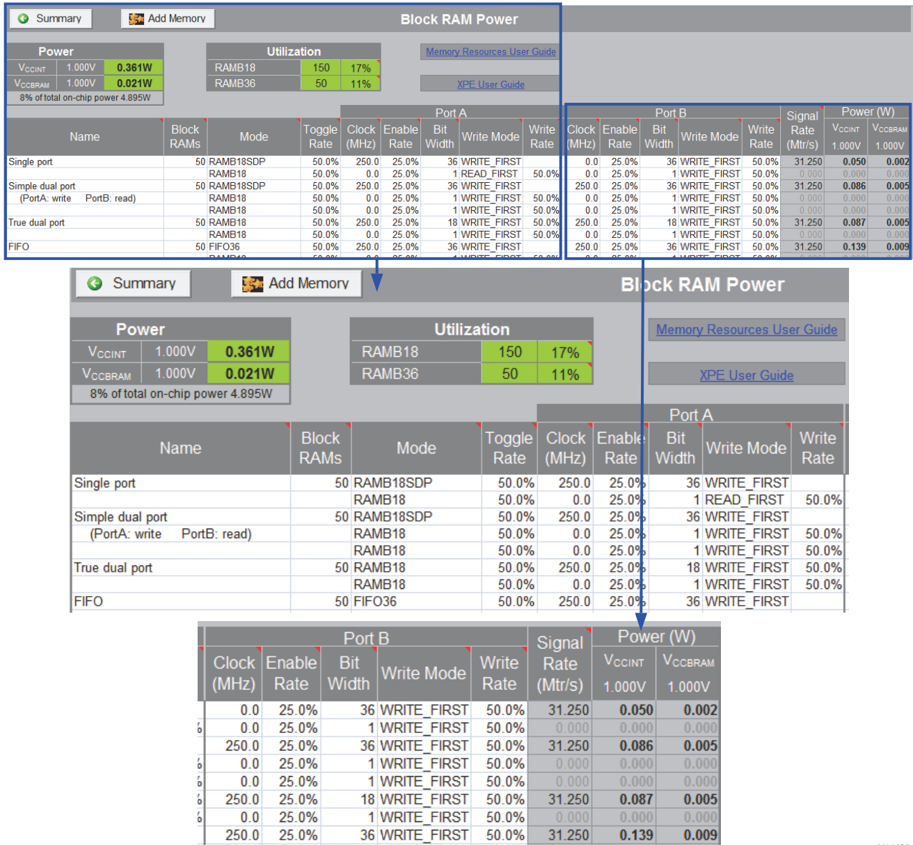
Figure 3-7: Block RAM Sheet - Effect of Block RAM Configuration Modes and Bit Widths on Power Estimates (7 Series Devices)
