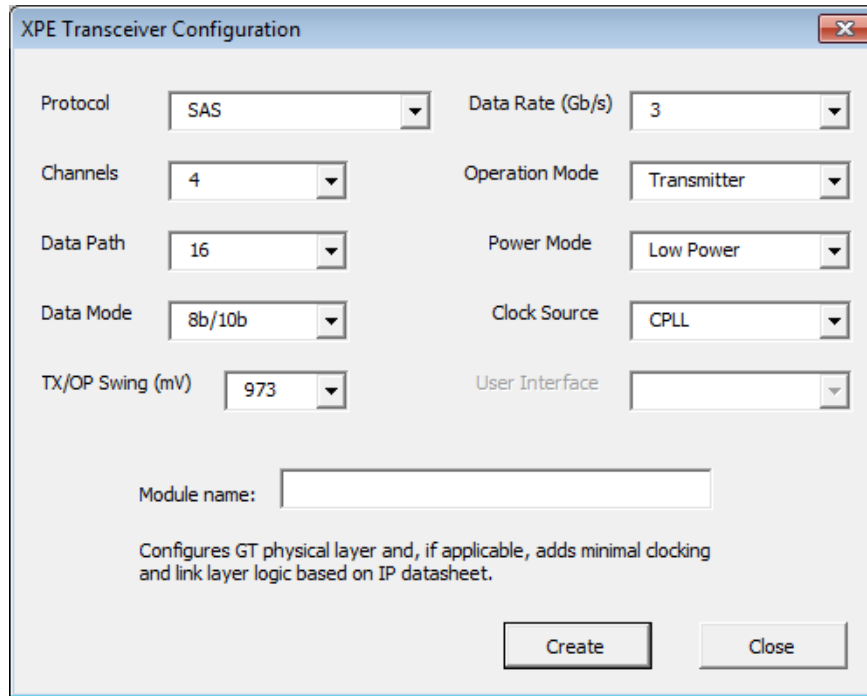
Figure 1-14: XPE Transceiver Configuration Dialog Box (Virtex-7 Devices)
