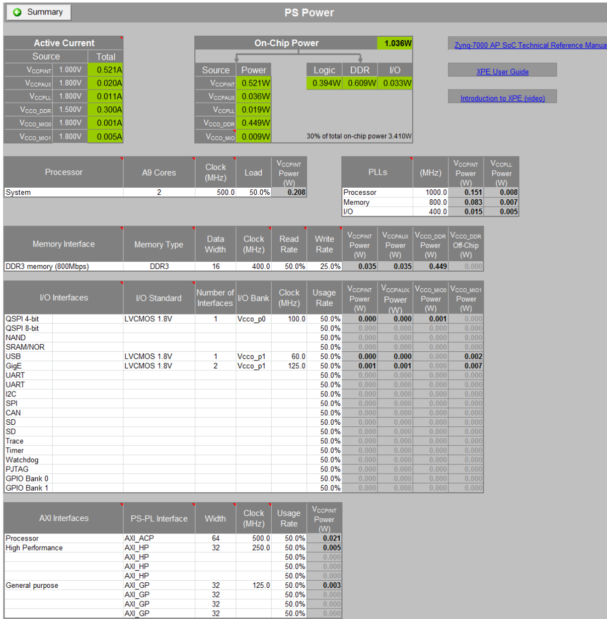
Figure 3-14: PS Power Sheet (Zynq-7000 AP SoC)
