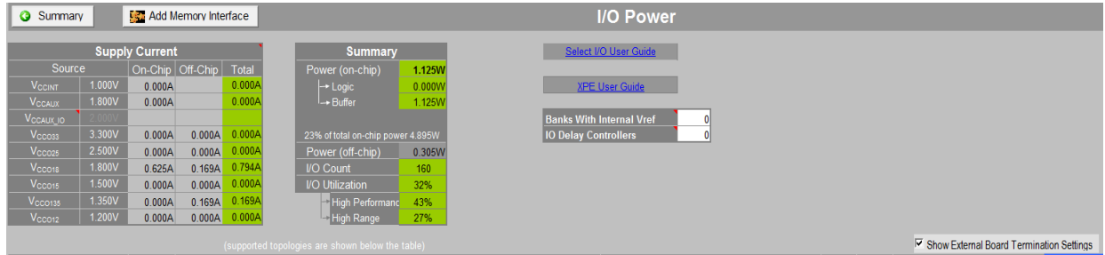
Figure 3-4: I/O Sheet - Top Section (7 Series Devices)
