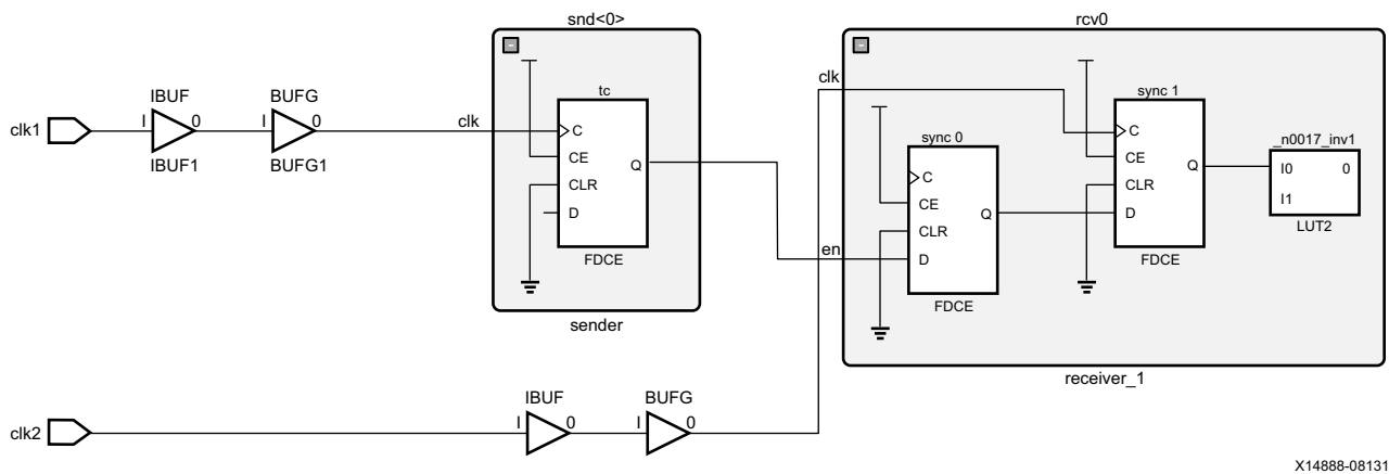
Figure 3-1: Synchronizing Clock Domains
