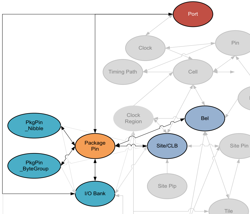
Figure 2-31: PACKAGE_PIN Objects
