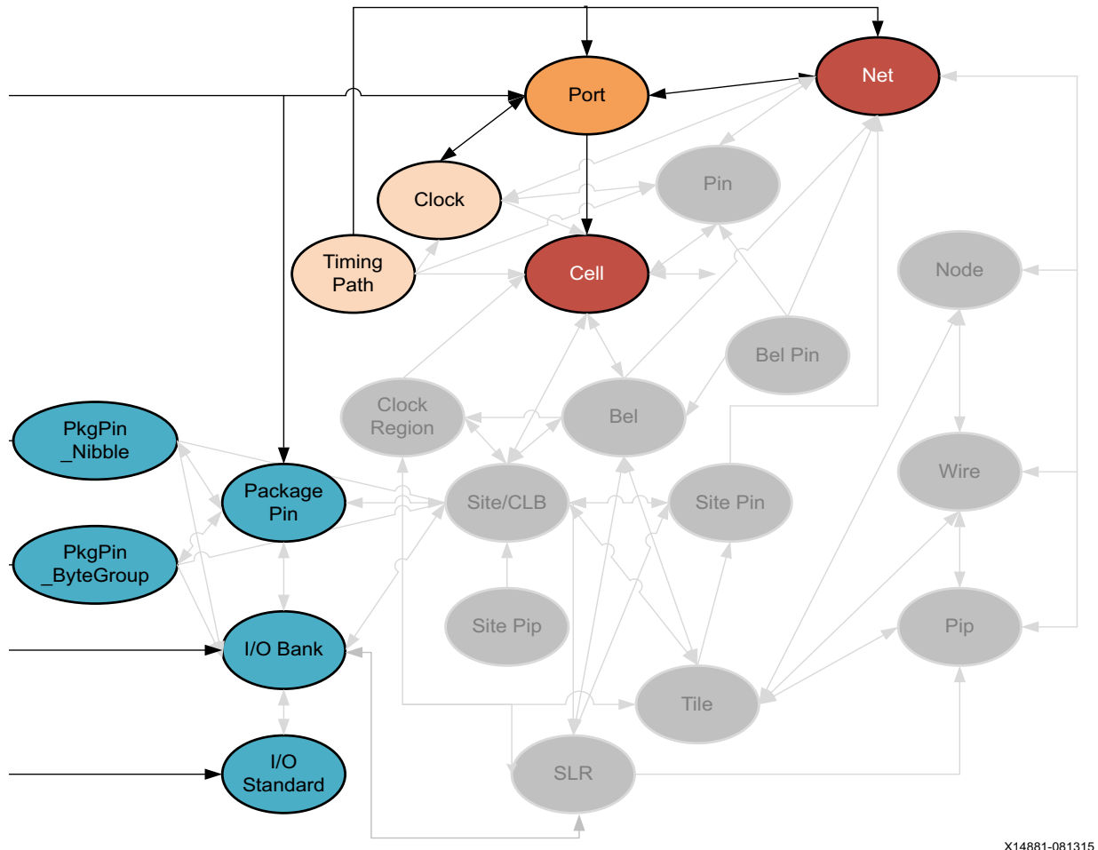
Figure 2-36: PORT Objects
