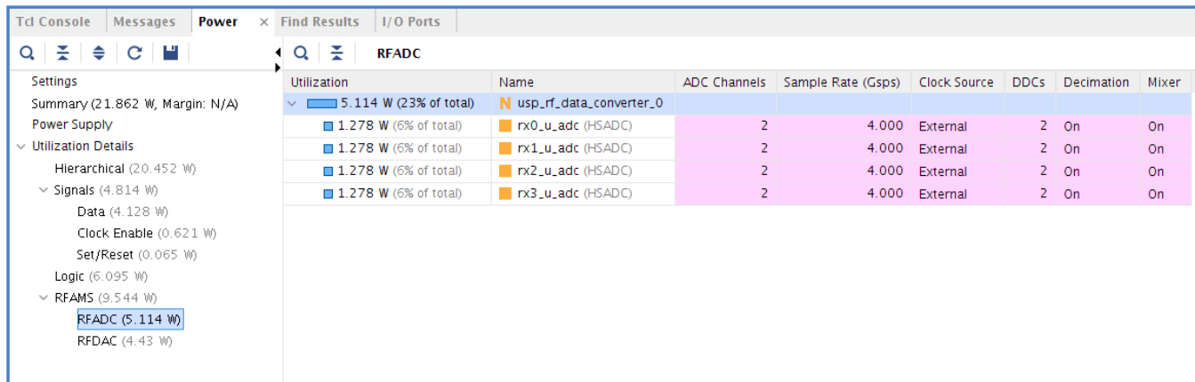
Figure 3-7: Report Power for RFADC
