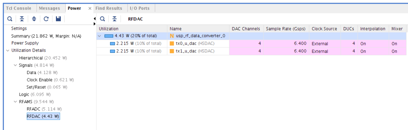
Figure 3-8: Report Power for RFDAC
