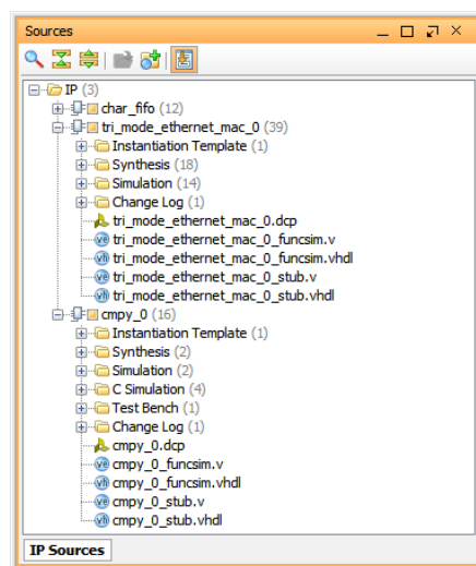
Figure 33: Output products of an IP
