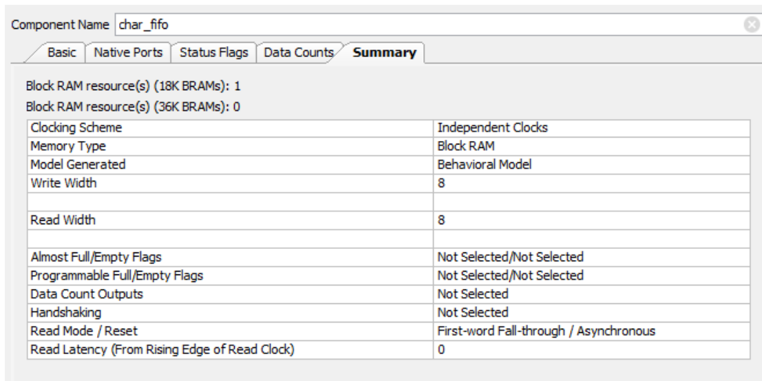
Figure 7: Summary of FIFO Generator Core
