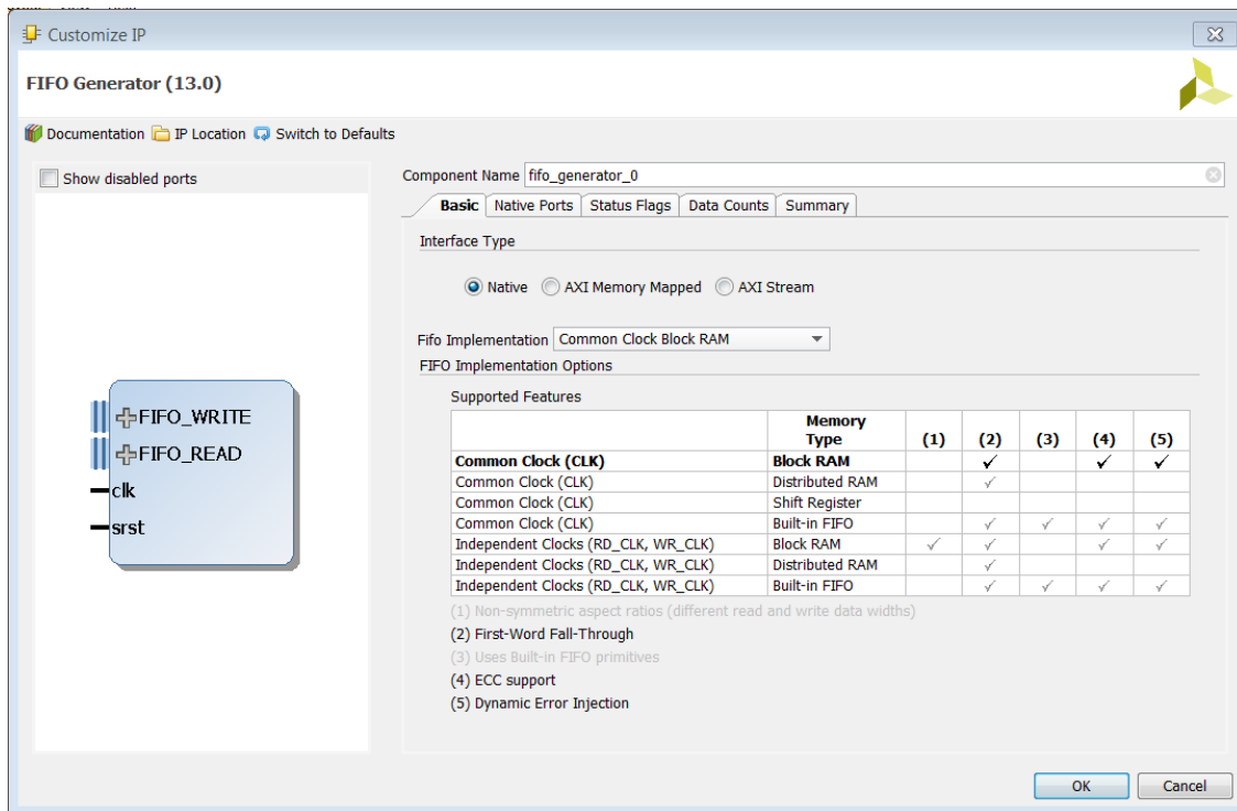
Figure 22: Customize IP Window
