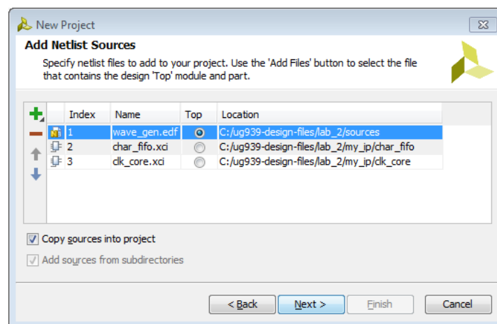
Figure 37: Add Sources to Netlist Project
