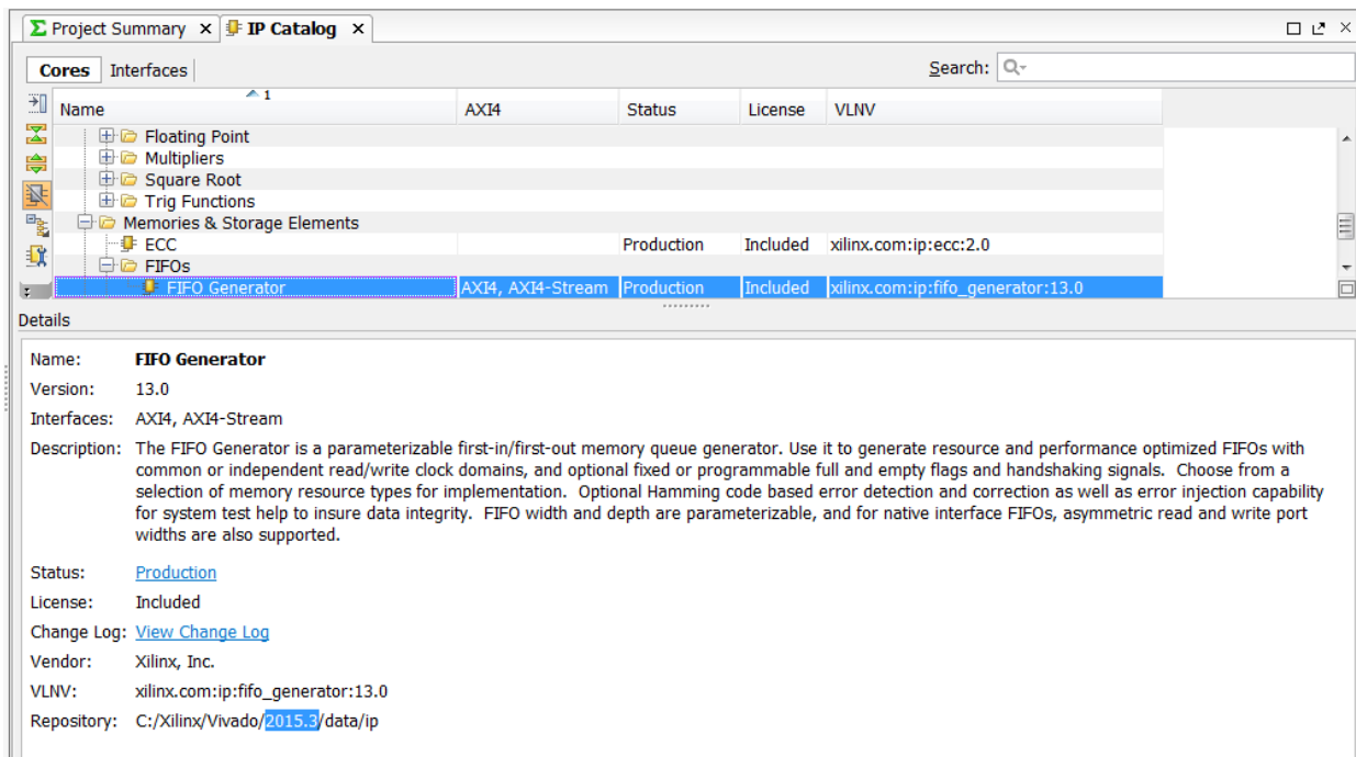
Figure 5: Xilinx IP Catalog – FIFO Core
