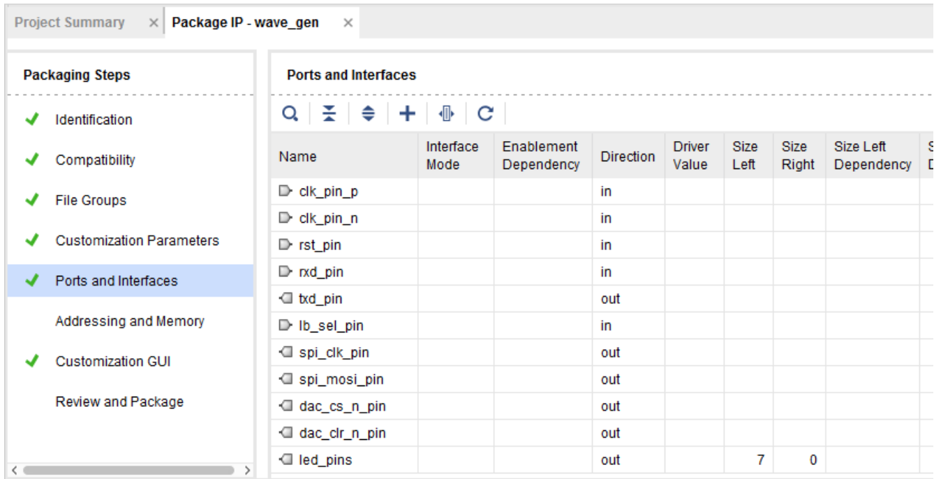
Figure 4-16: Package IP – Ports and Interfaces
