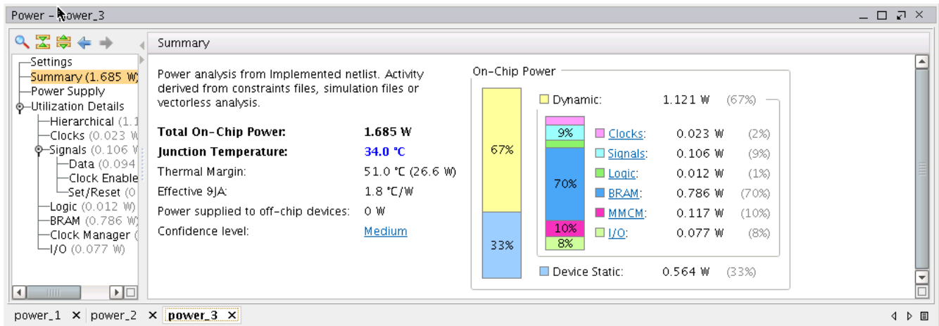
Figure 59: Power Report – Vectorless Analysis with Junction Temperature Supplied
