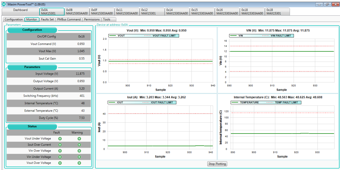
Figure 67: Monitoring a Rail - Voltage and Current
