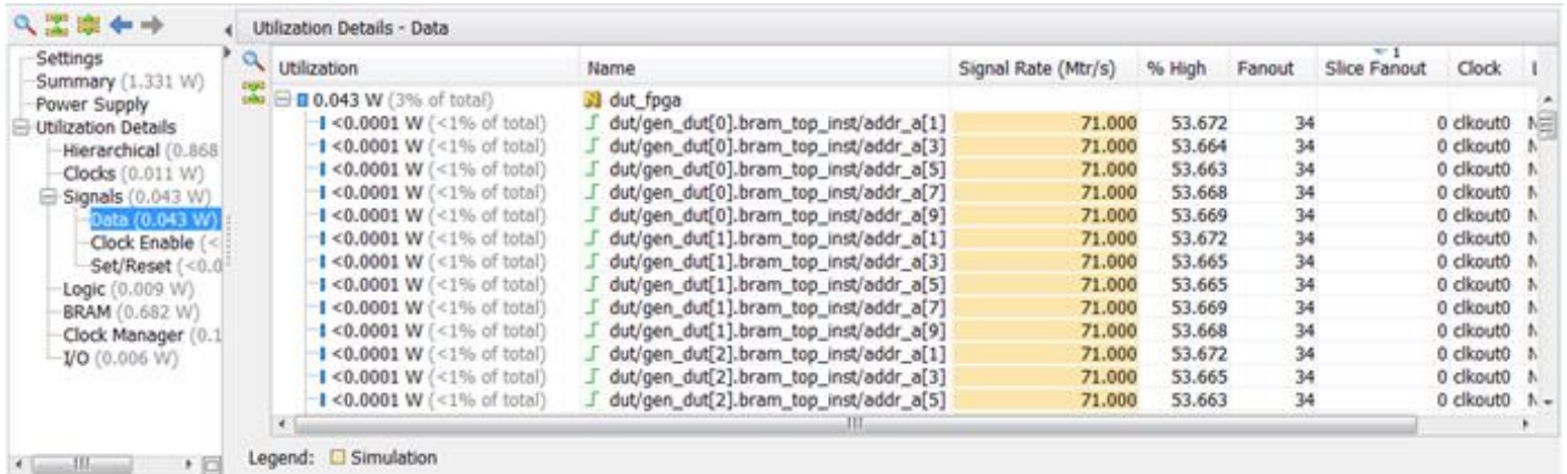
Figure 47: Signals > Data View with SAIF File Data
