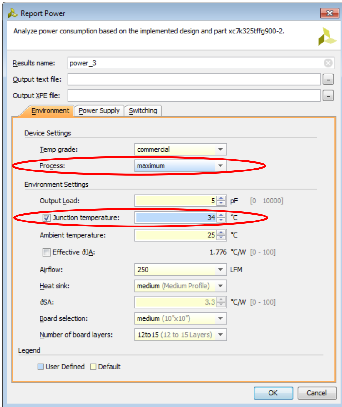
Figure 58: Report Power Settings – Updating Junction Temperature
