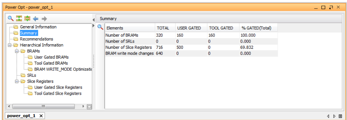
Figure 75: Power Optimization Report – Tool Gated BRAMs
