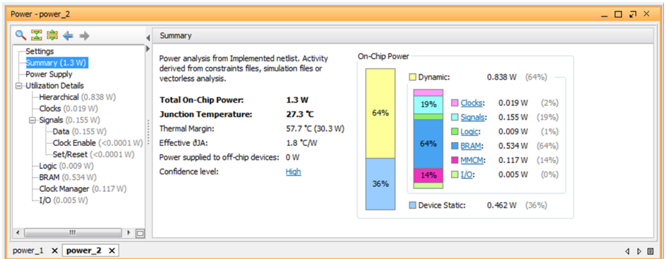
Figure 35: Power Report with SAIF Data
