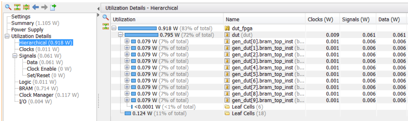
Figure 12: Power Report – Hierarchical Display
