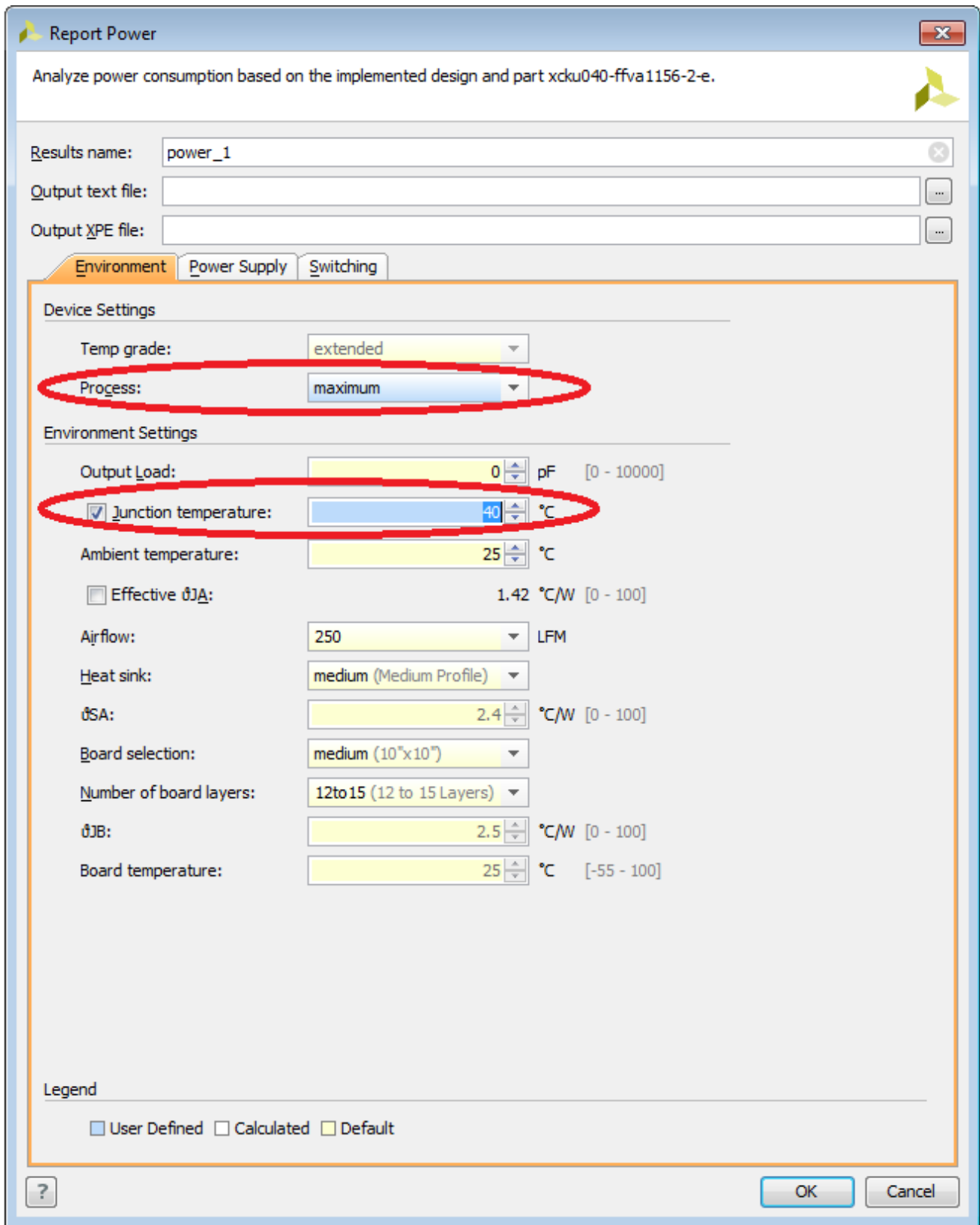
Figure 68: Reporting Power Settings – Updating Junction Temperature
