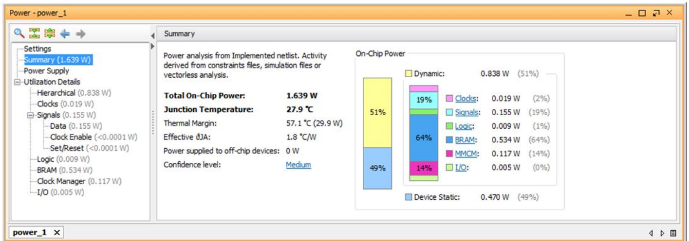
Figure 45: Power Report – Vectorless Mode Run
