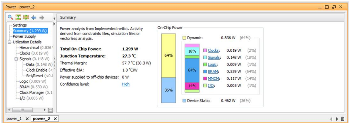
Figure 46: Power Report – With SAIF File Data
