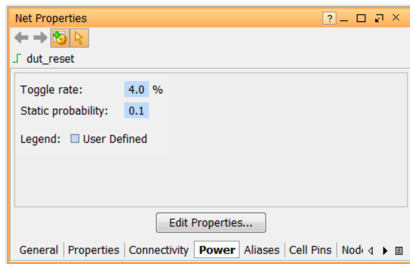
Figure 17: User Defined Color in Net Properties Window
