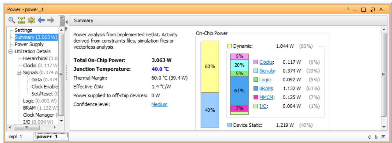
Figure 69: Power Report – Vector Analysis with Junction Temperature Supplied
