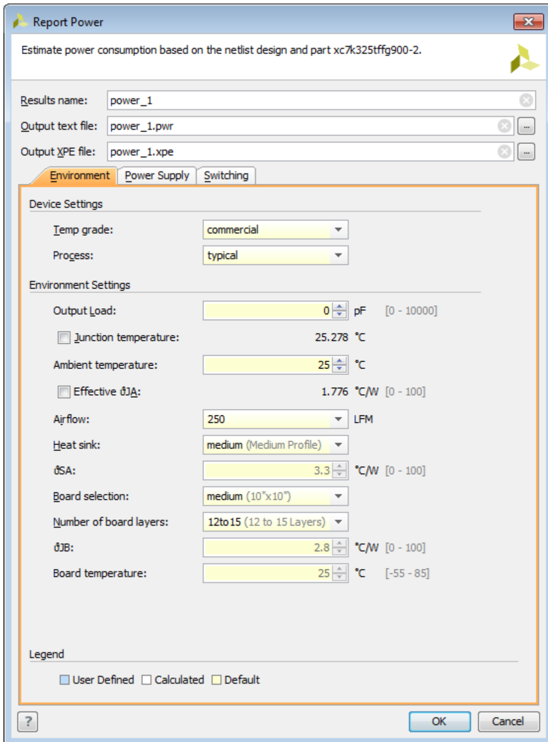
Figure 7: Report Power Dialog Box
