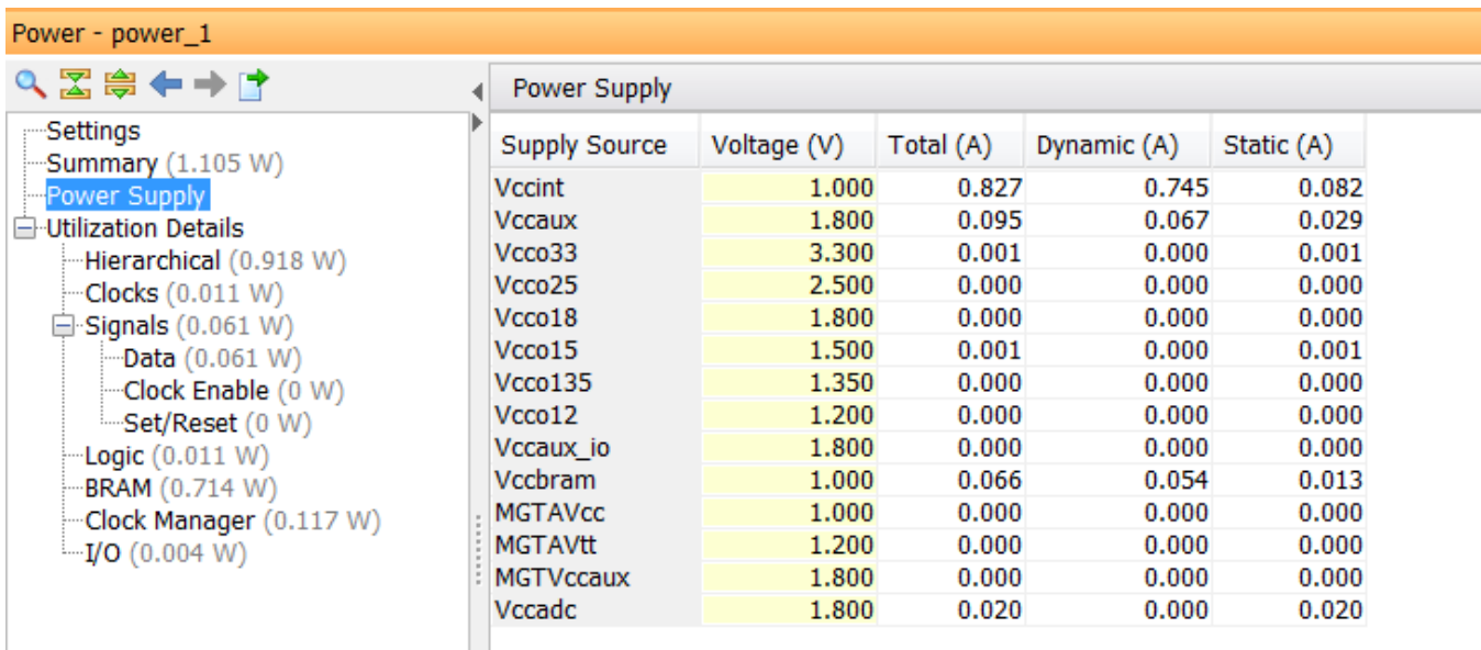
Figure 11: Power Report – Power Supply Display
