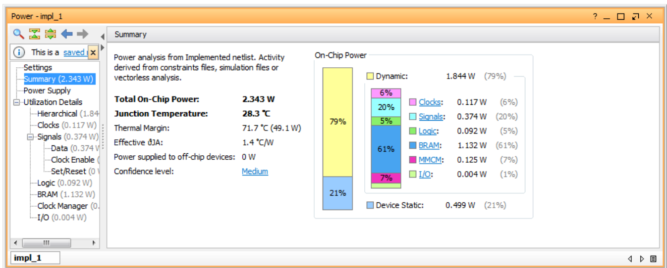
Figure 80: Power Report Summary
