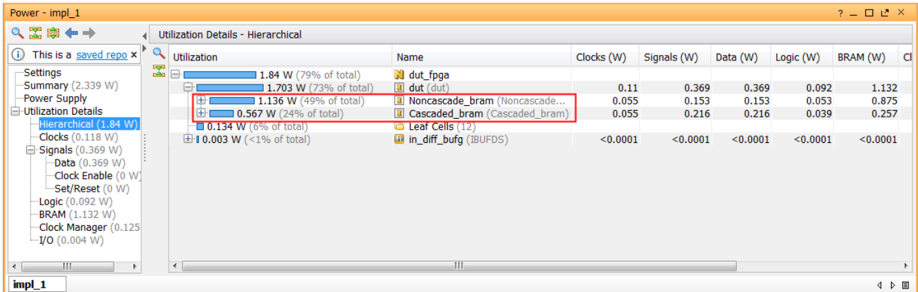
Figure 81: Cascaded and Non Cascaded BRAM Power view
