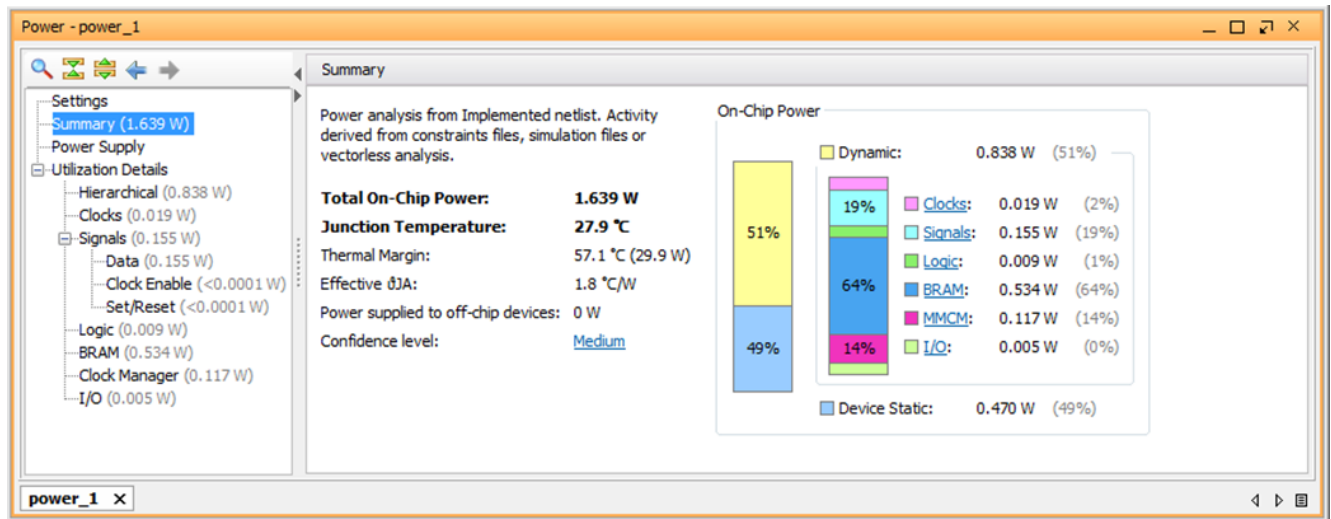
Figure 34: Running Post-Implementation Report Power in Vectorless Mode
