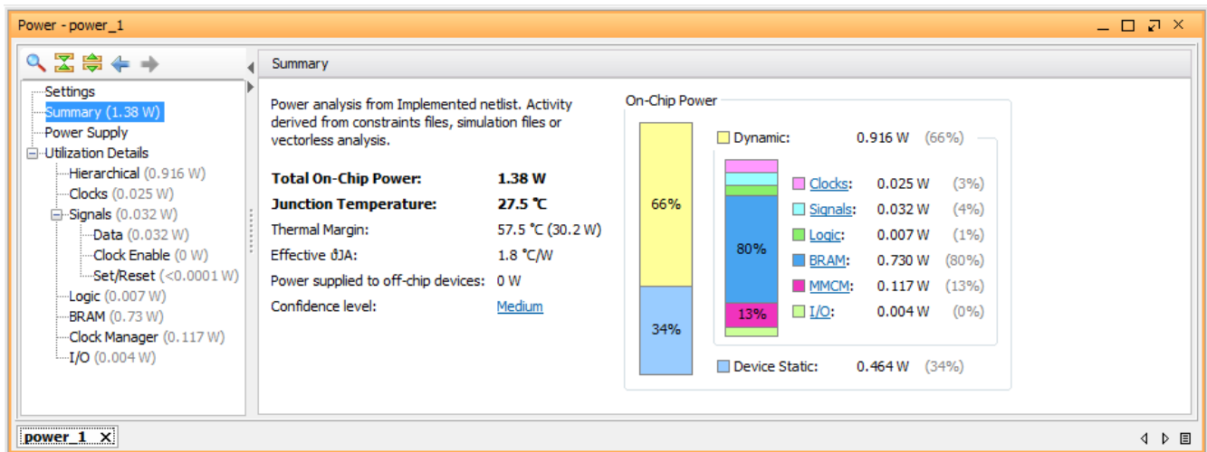
Figure 76: Power Savings with Power Optimization
