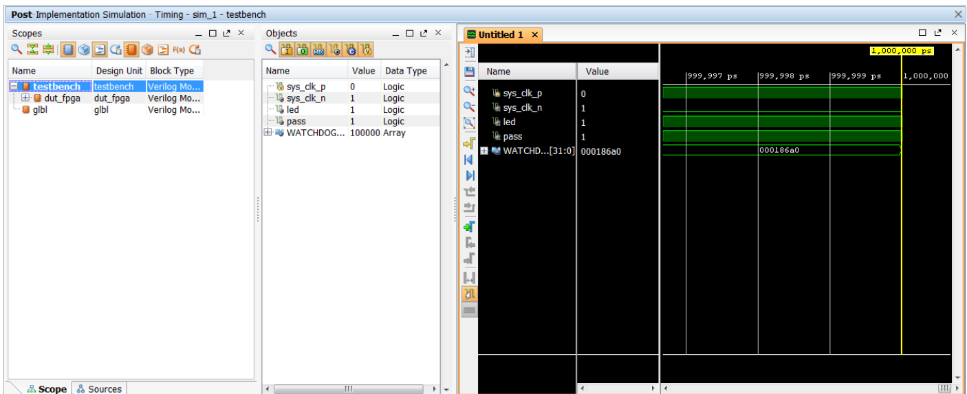
Figure 33: Post-Implementation Timing Simulation using the Vivado Simulator
