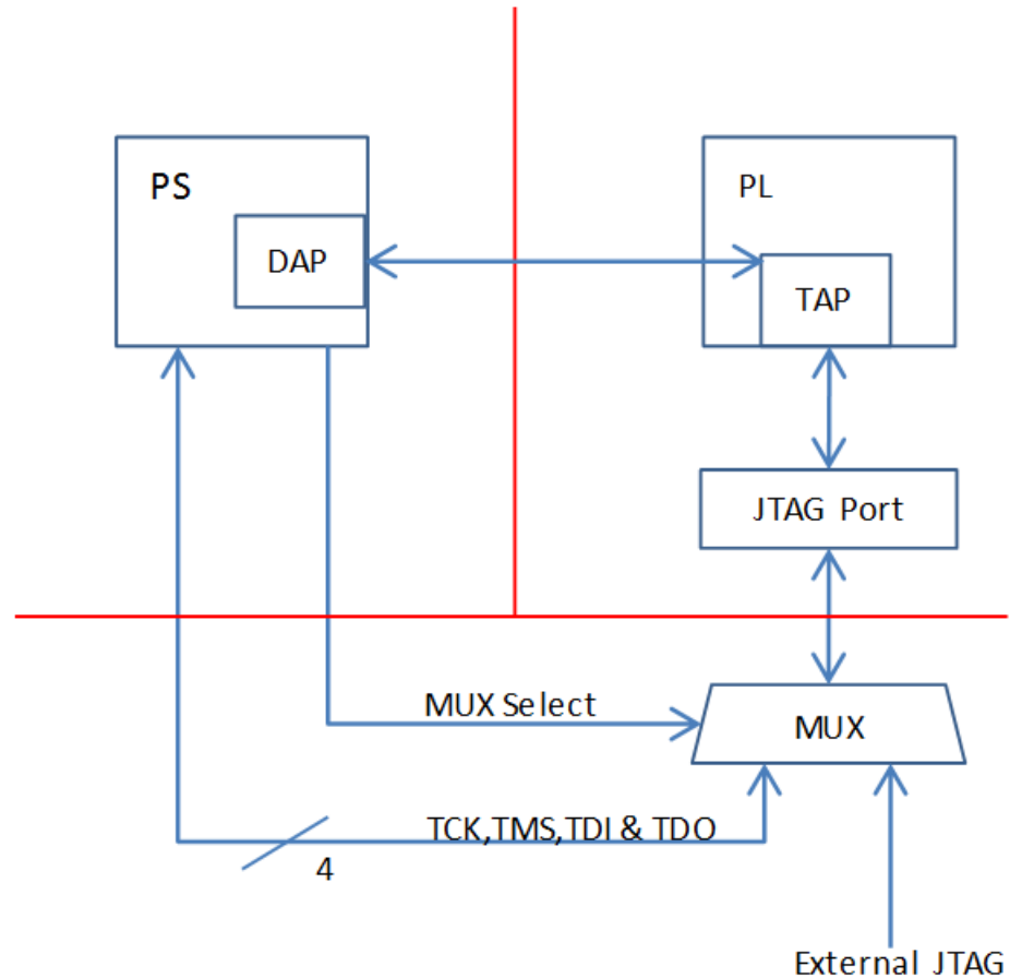
Figure 1: MUX Usage
