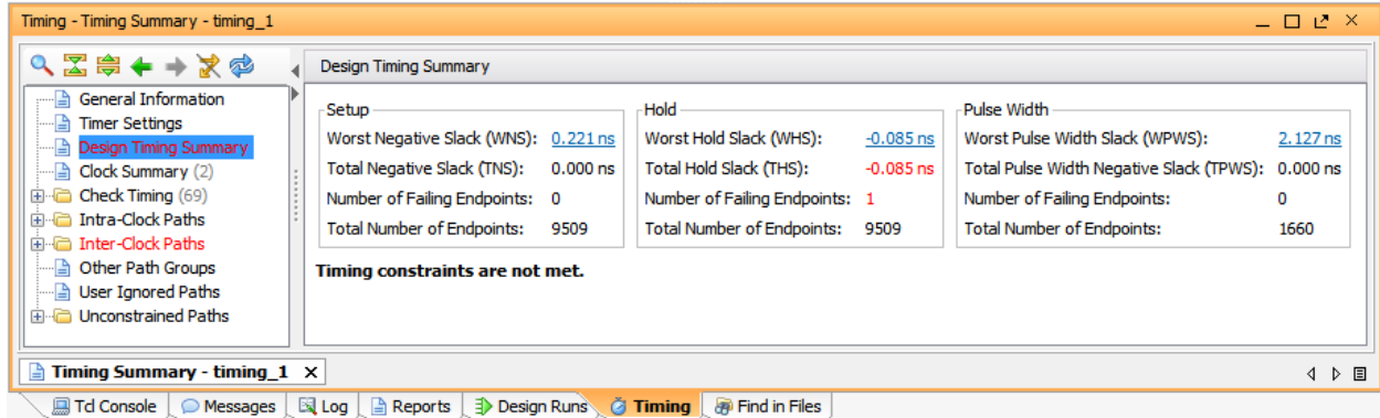
Figure 26: Report Timing Summary
