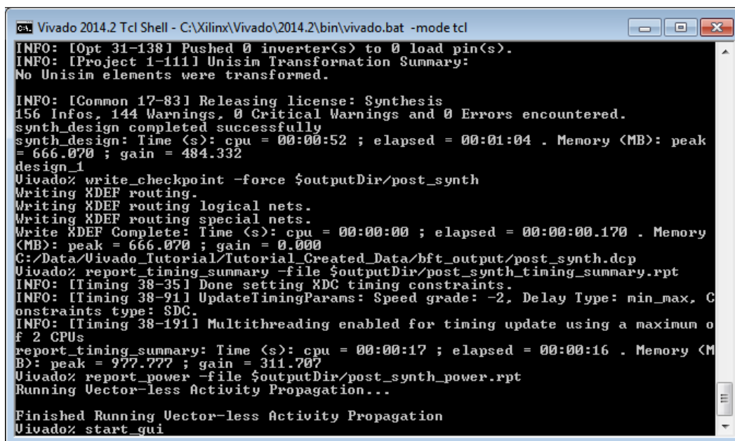
Figure 2: Open the Vivado IDE with start_gui
