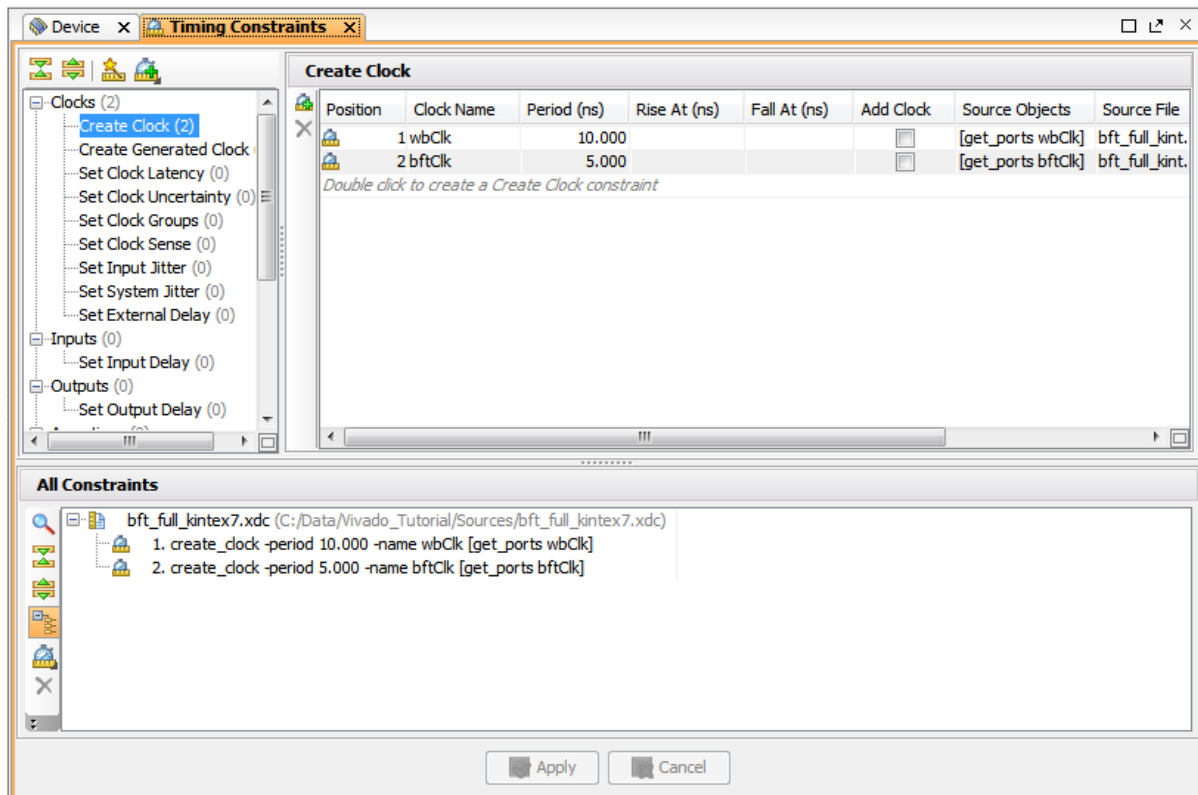
Figure 4: Define Timing Constraints
