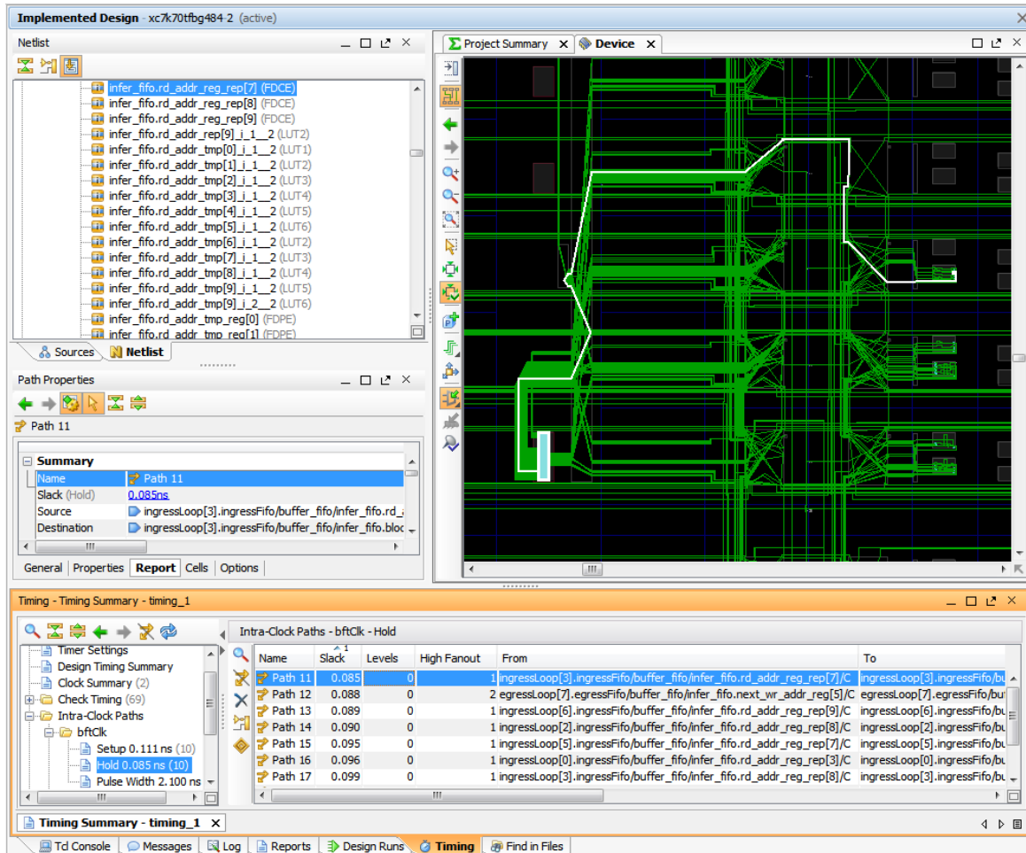
Figure 28: Examine Routing for Timing Paths
