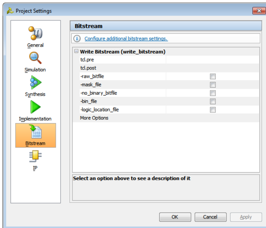
Figure 29: Bitstream Settings
