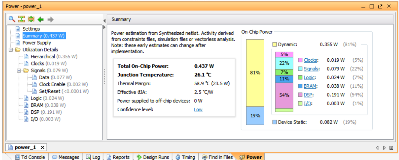
Figure 27: Report Power
