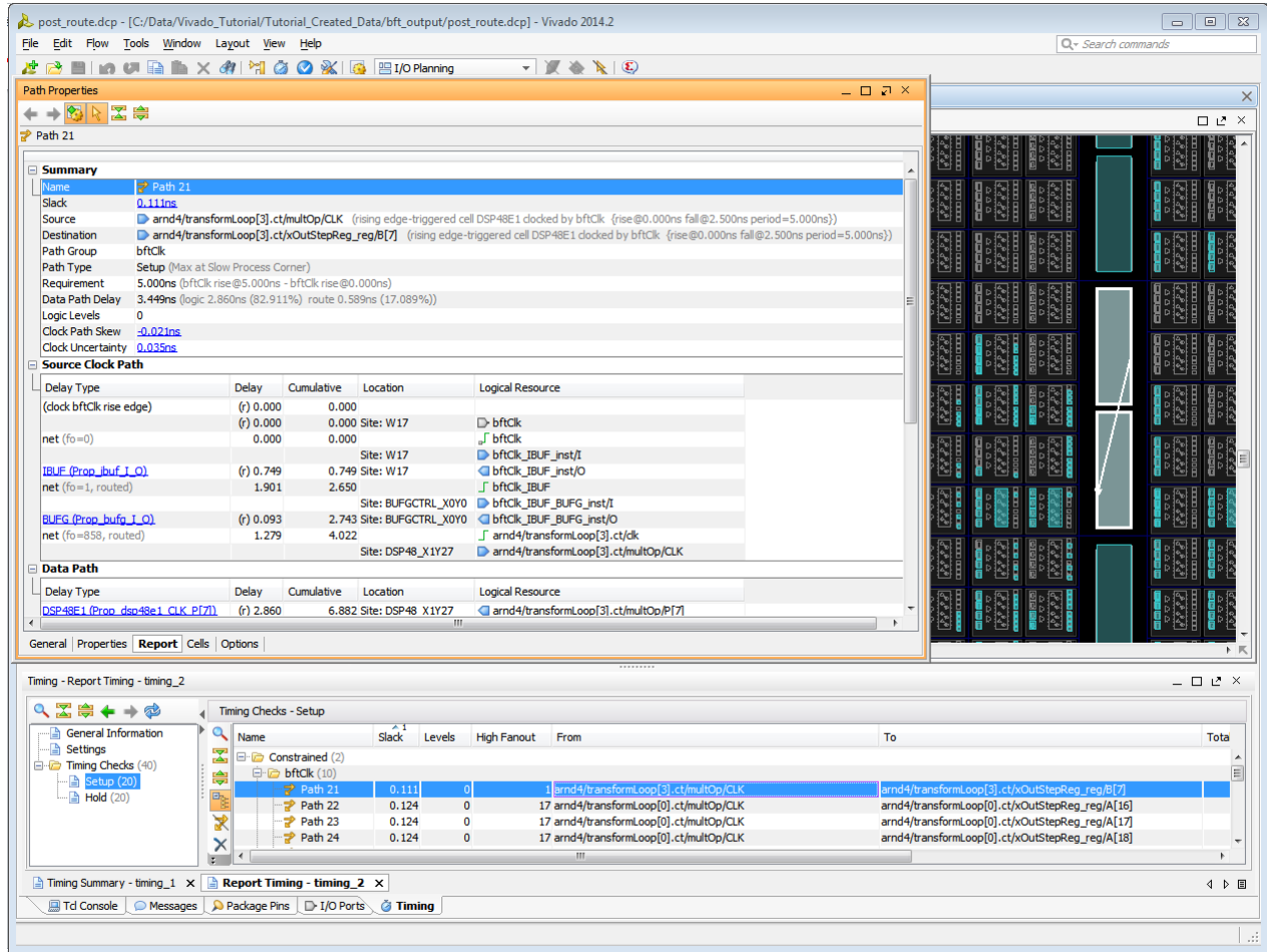
Figure 8: Float the Path Properties Window
