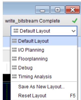
Figure 2-3: Layout Selector
