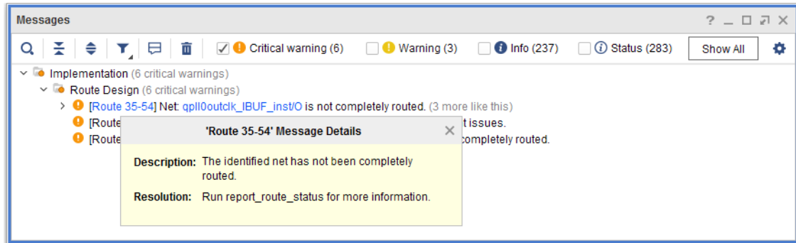
Figure 3-49: Message Details
