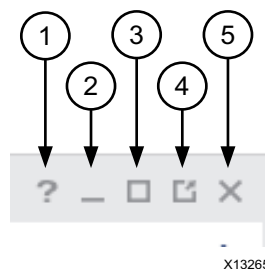
Figure 3-3: Window Controls
