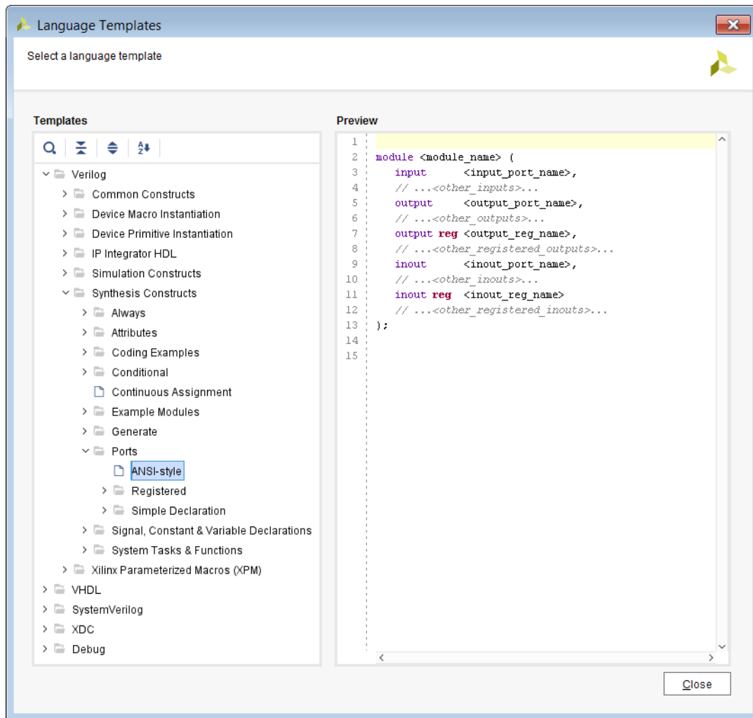
Figure 2-6: Language Templates
