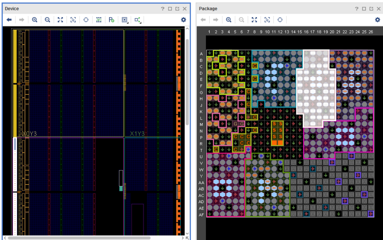
Figure 3-25: Vertically Tiled Windows
