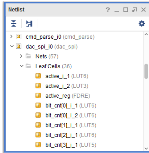
Figure 3-16: Netlist Window Leaf Cells Folder
