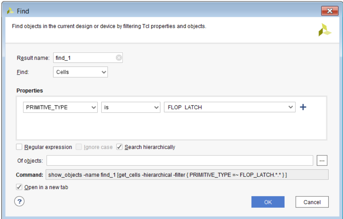
Figure 2-9: Find Dialog Box
