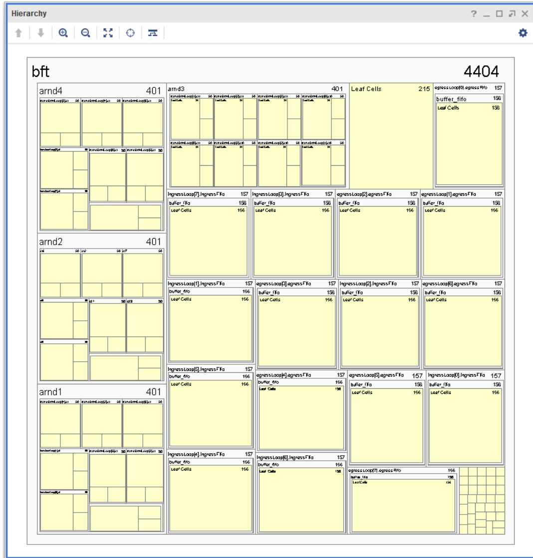
Figure 3-42: Hierarchy Window Block View
