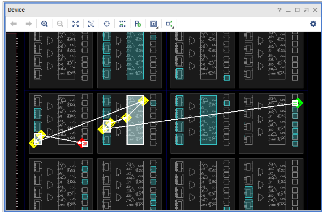
Figure 3-22: Marked Timing Path Symbols in Device Window
