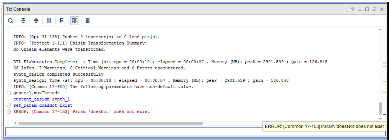
Figure 3-46: Warnings and Errors in the Tcl Console
