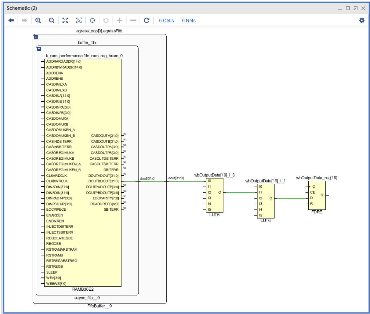
Figure 3-40: Timing Path in Schematic Window
