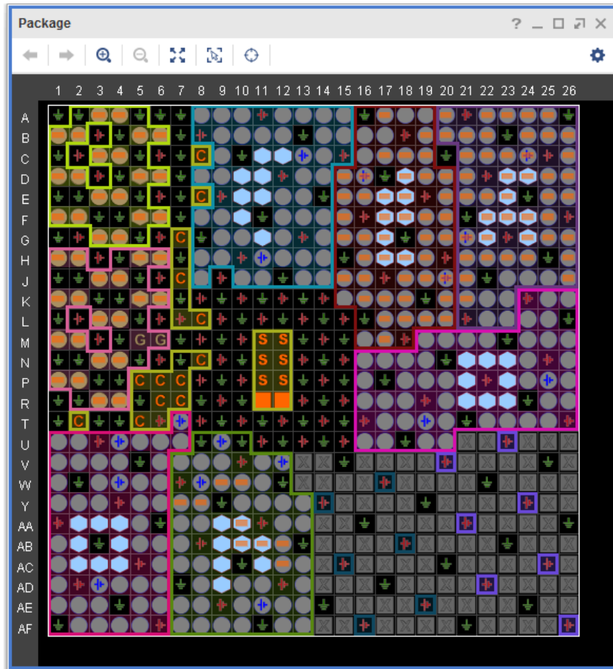
Figure 3-32: Package Window
