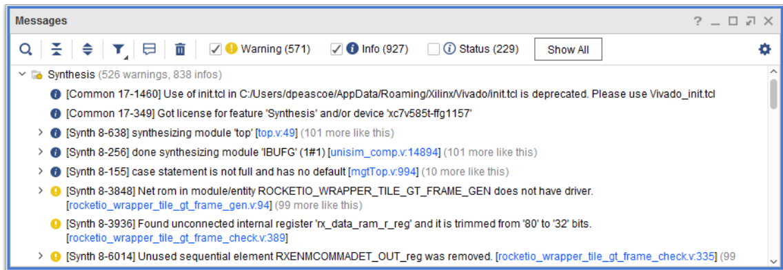
Figure 3-48: Messages Window
