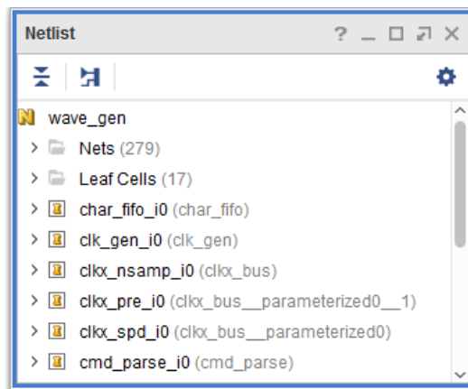
Figure 3-15: Netlist Window
