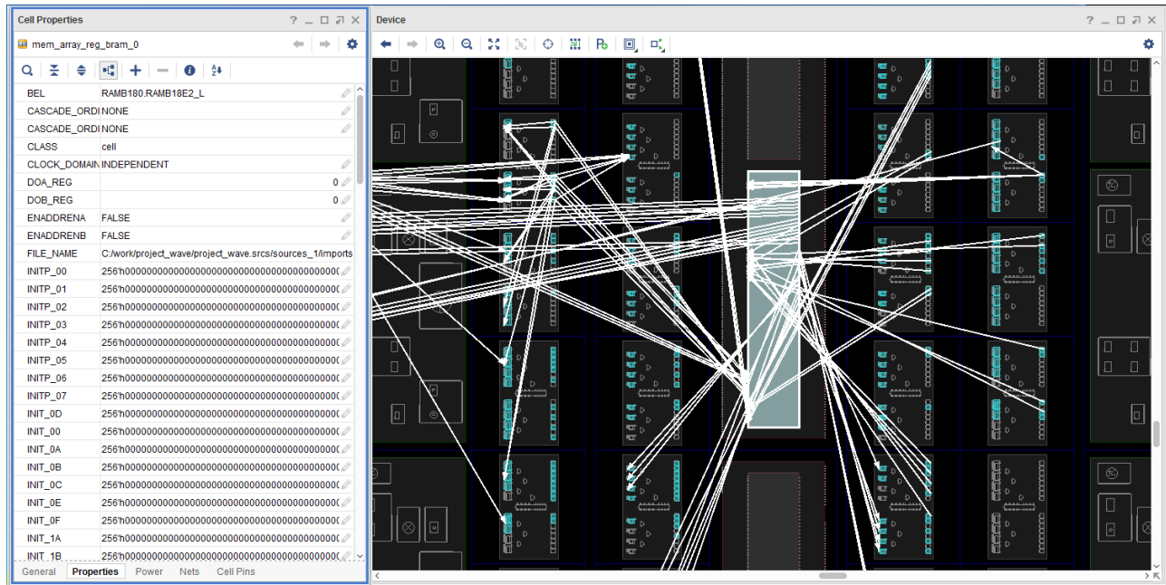
Figure 3-19: Properties Window
