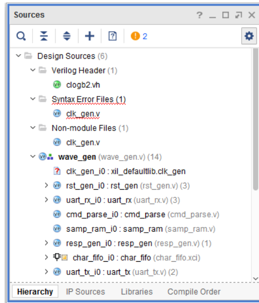
Figure 3-12: Sources Window
