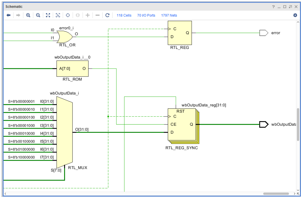
Figure 3-41: RTL Schematic with Bundled Logic
