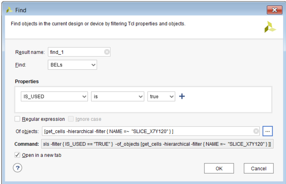
Figure 2-14: Finding Occupied BELs within a Slice
