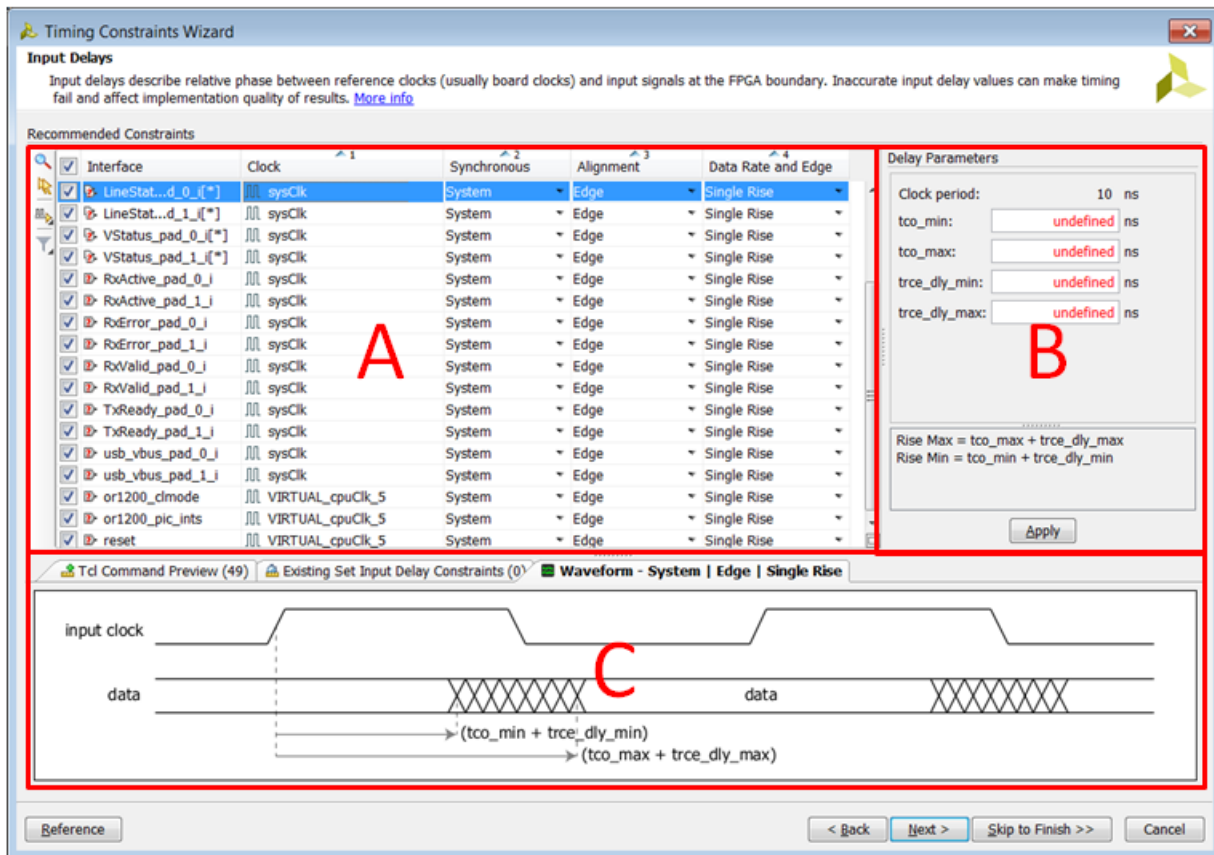
Figure 12: Input Delay Page of Timing Constraints Wizard Showing the Major Sections
