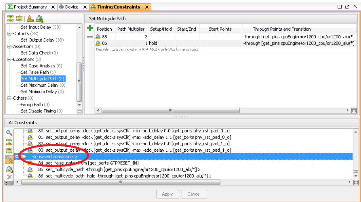
Figure 21: Unsaved Constraints Displayed in the Constraints Editor.
