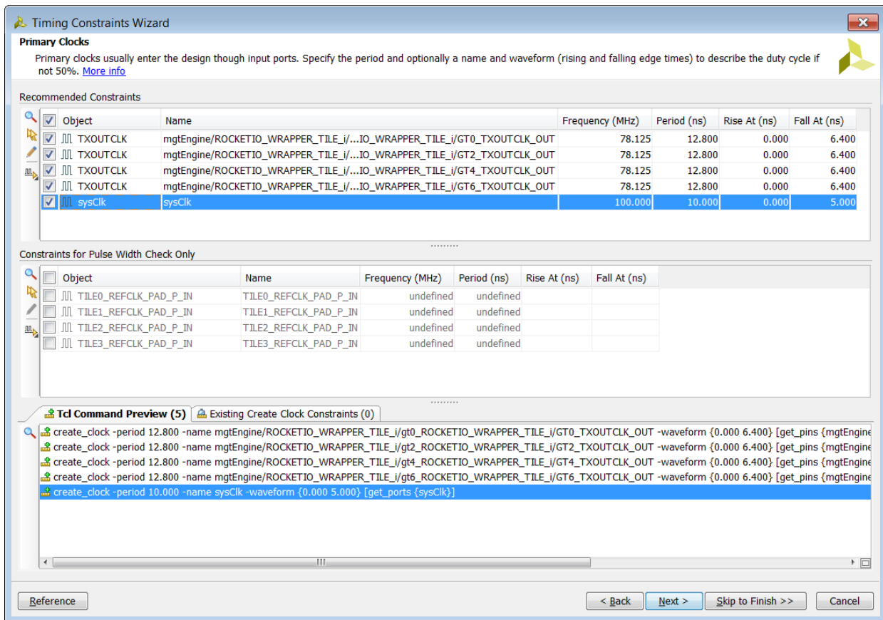
Figure 11: Completed Primary Clocks Page of the Timing Constraints Wizard
