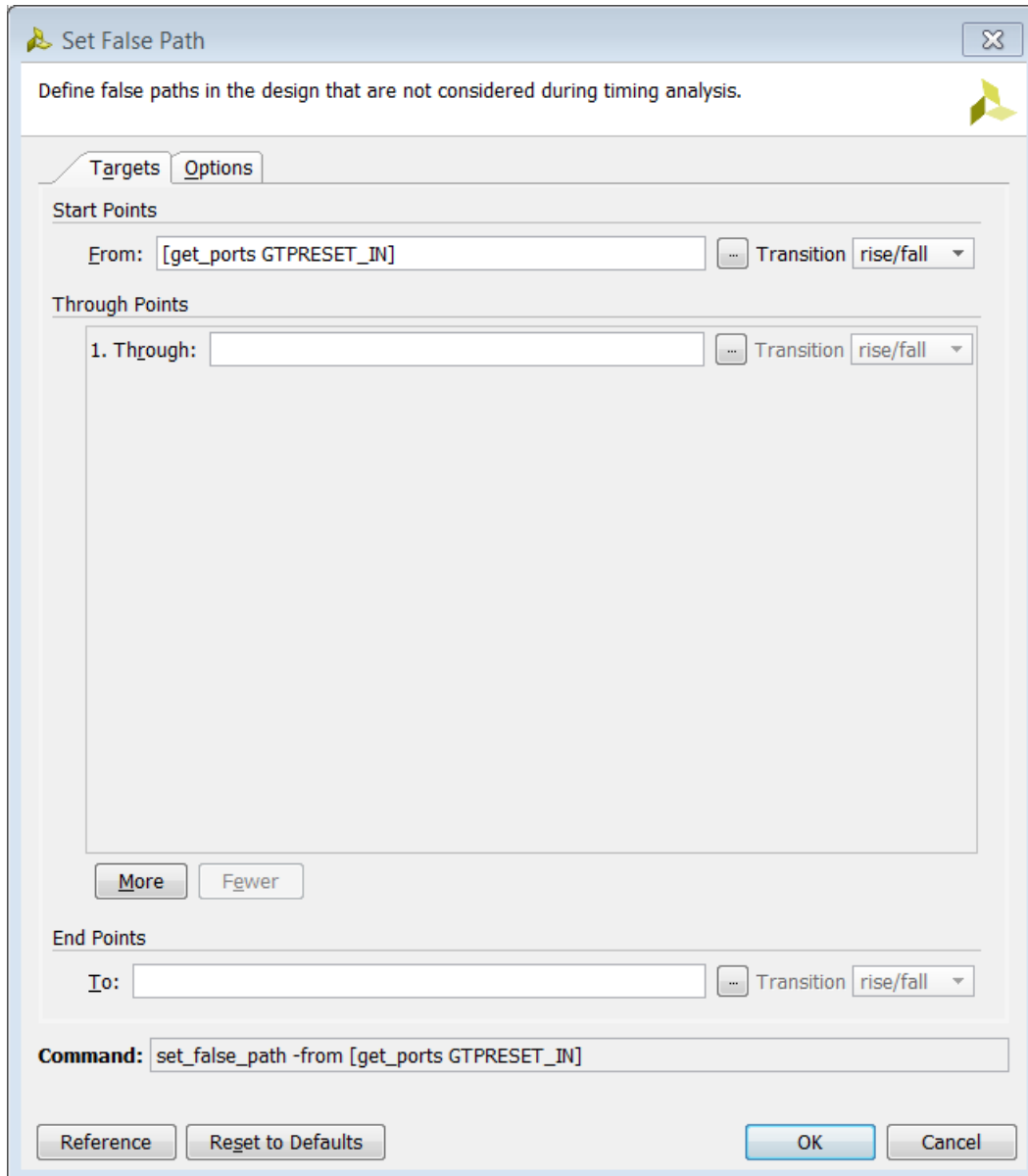
Figure 18: Completed set_false_path Constraint Window
