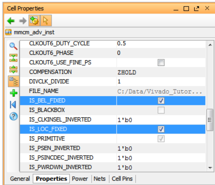
Figure 32: BEL and LOC Placement Constraints
