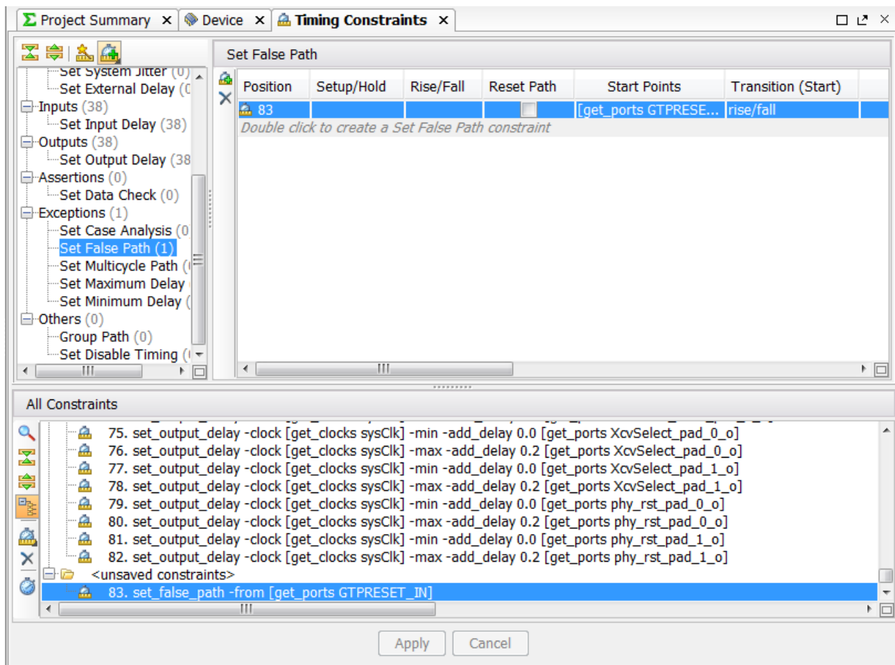
Figure 19: New set_false_path constraint in the Constraints Editor
