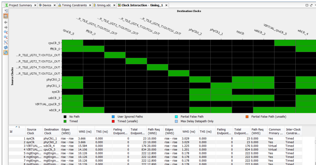
Figure 23: Clock Interaction Report
