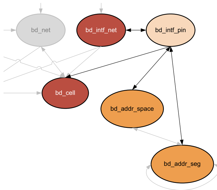
Figure 2-5: Block Design Interface Pin
