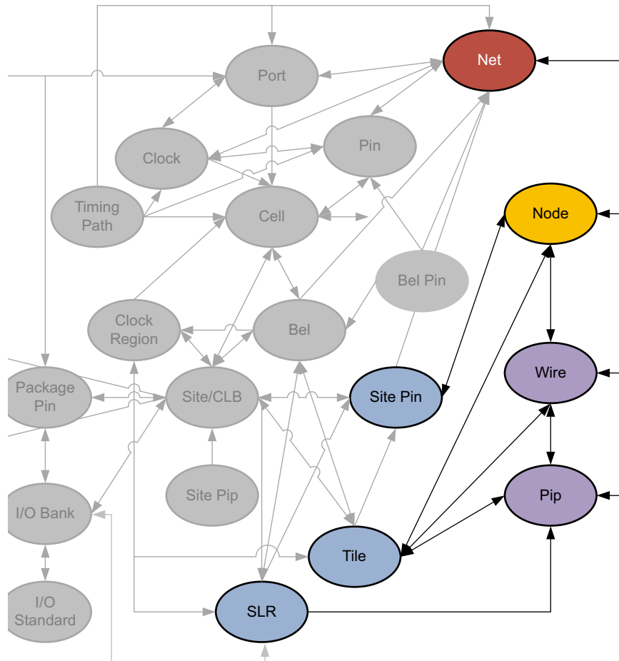
Figure 2-30: NODE Objects
