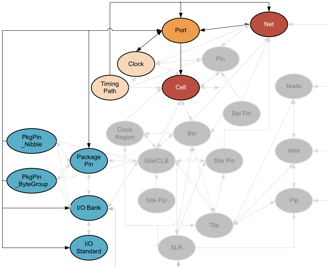
Figure 2-36: PORT Objects
