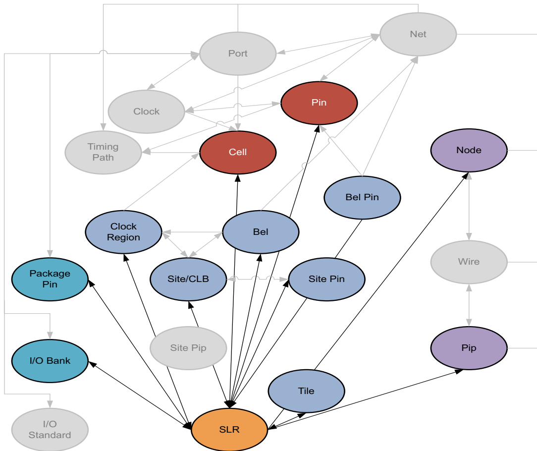
Figure 2-38: SLR Objects
