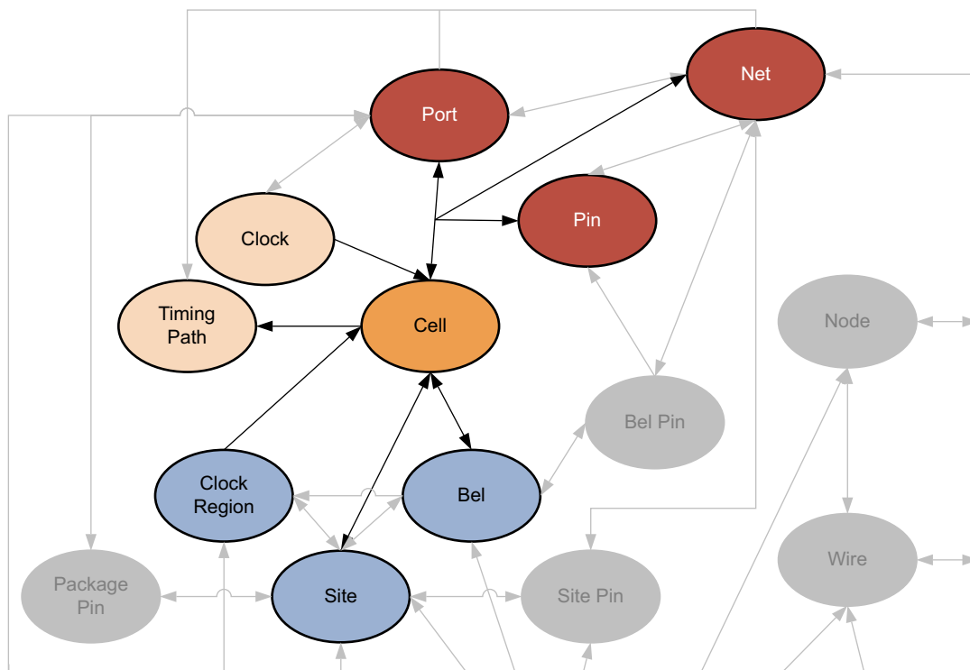
Figure 2-12: CELL Objects
