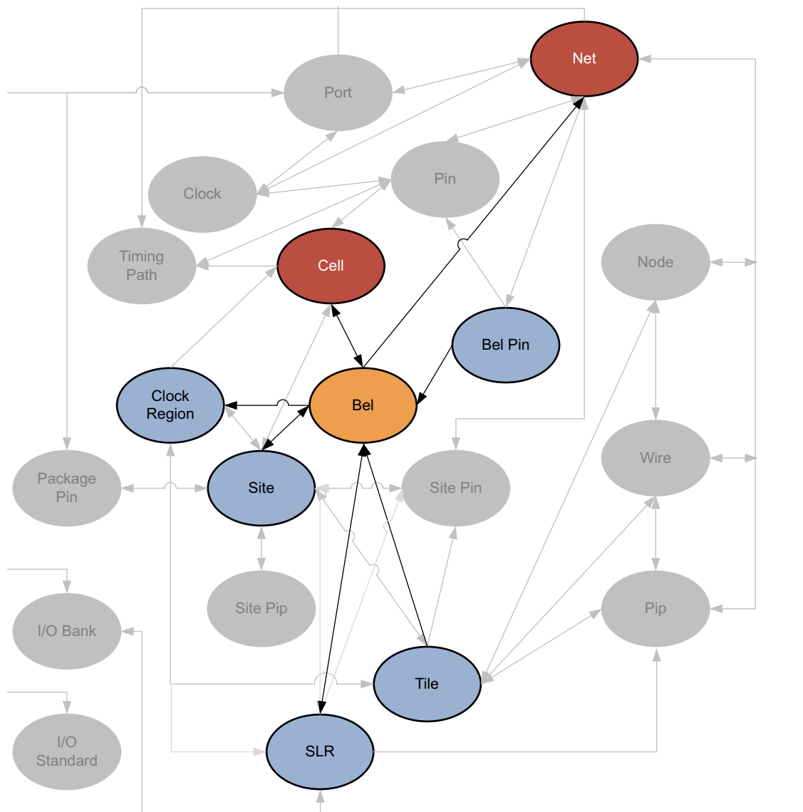
Figure 2-10: BEL Objects
