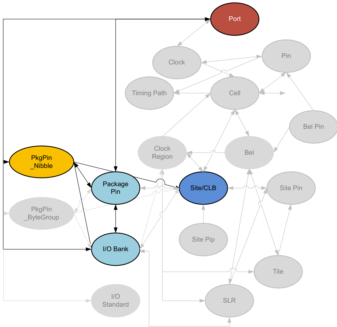
Figure 2-35: PKGPIN_NIBBLE Objects
