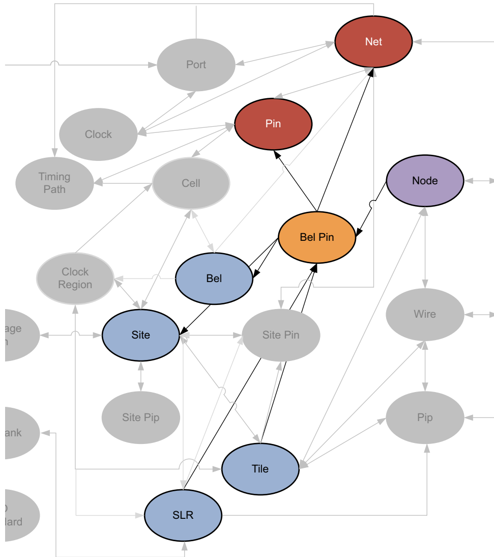
Figure 2-11: BEL_PIN Objects
