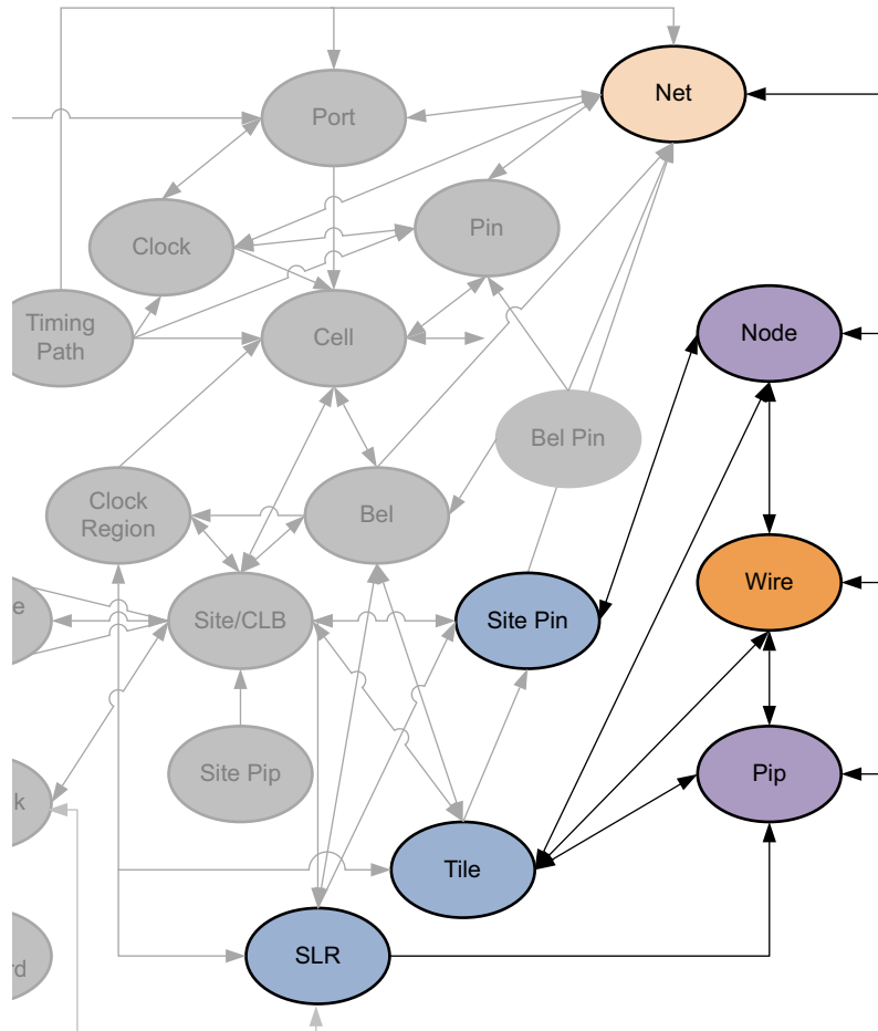
Figure 2-41: WIRE Objects
