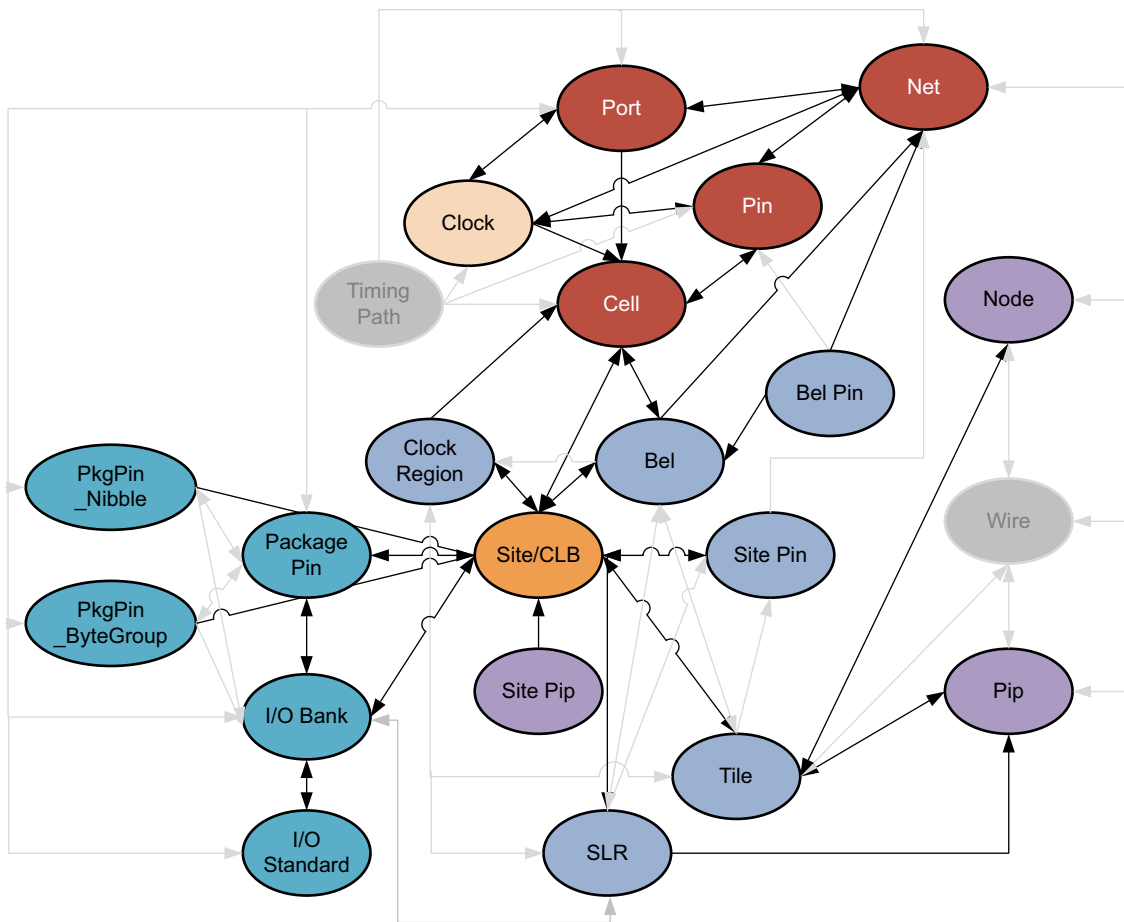
Figure 2-37: SITE Objects
