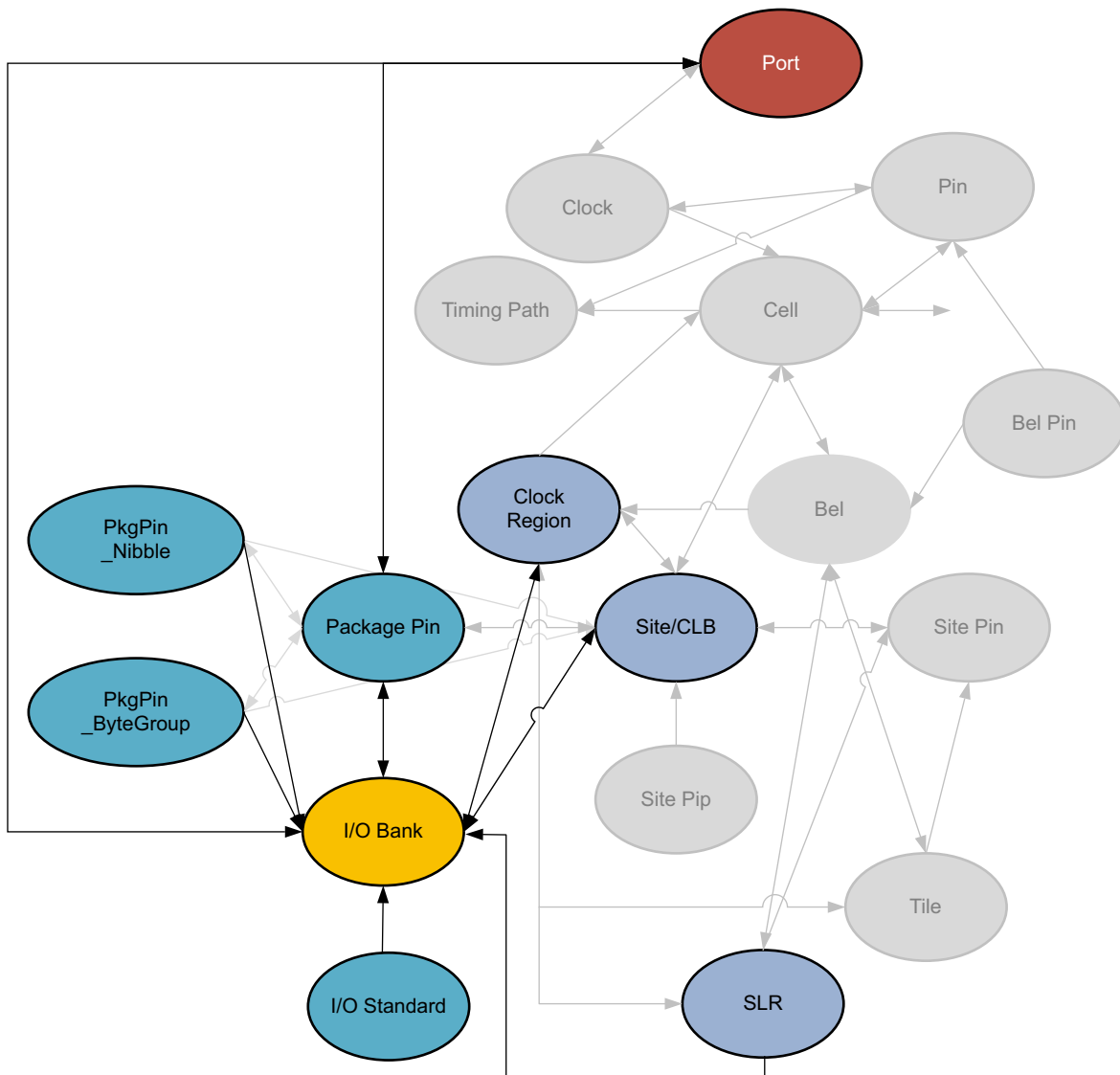
Figure 2-27: IO_BANK Objects
