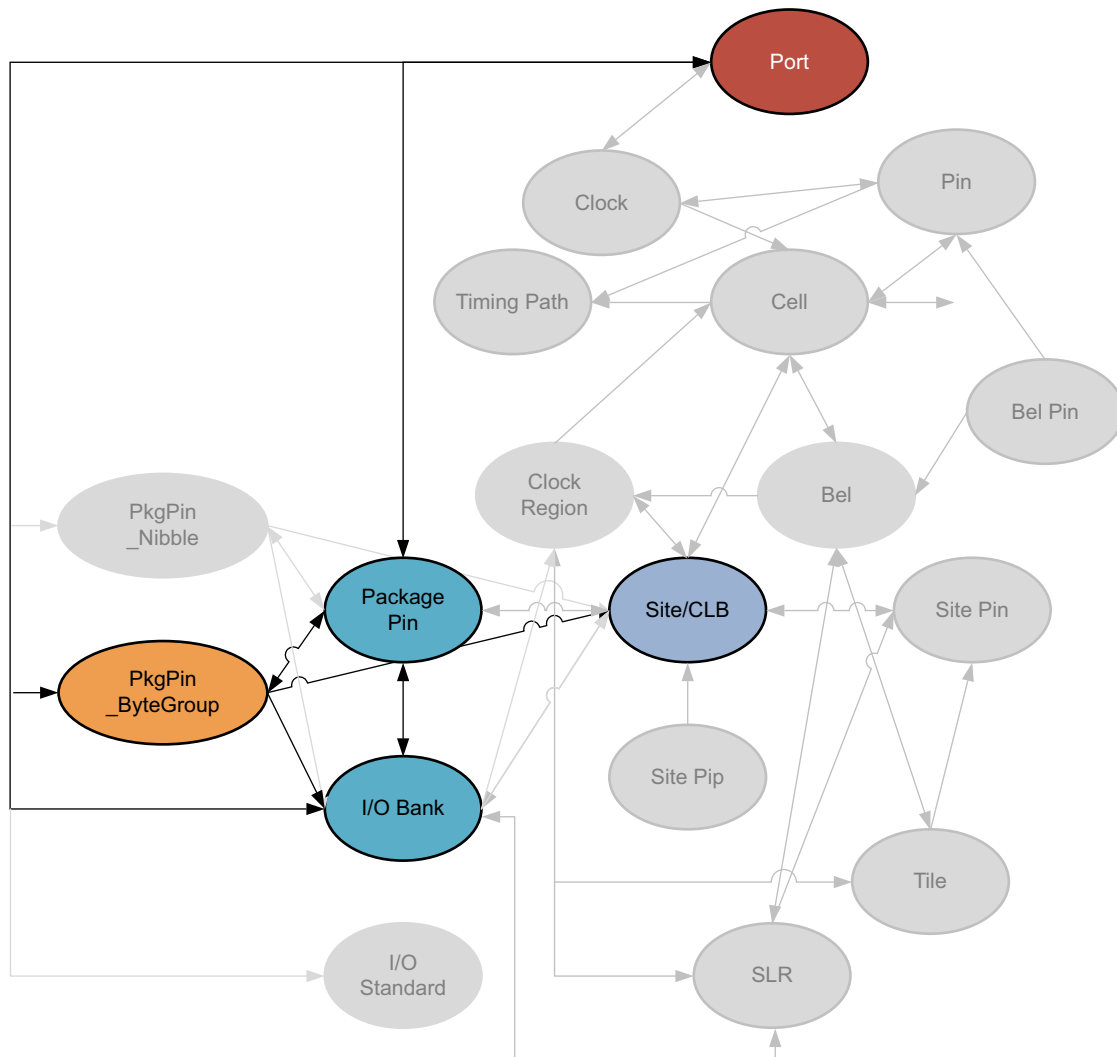
Figure 2-34: PKGPIN_BYTEGROUP Objects
