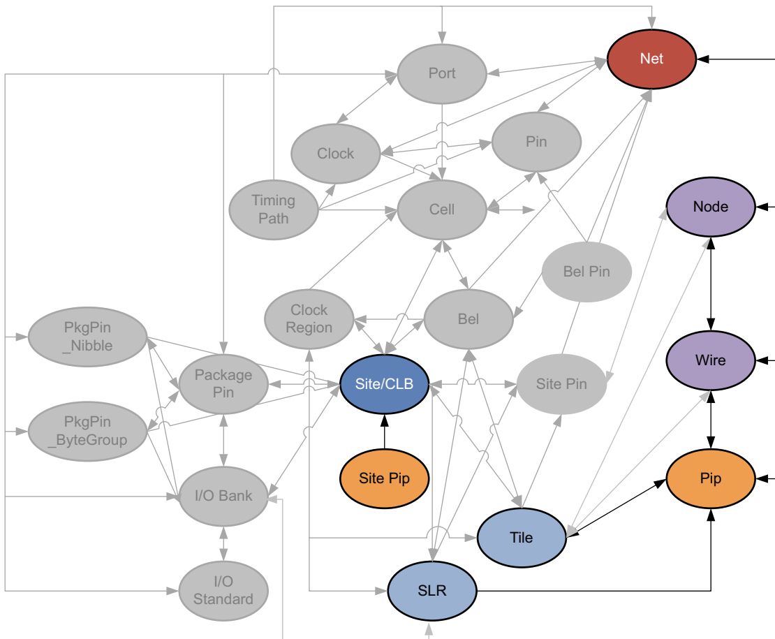
Figure 2-33: PIP Objects
