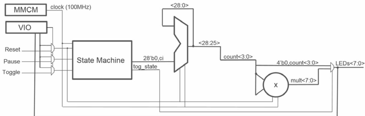
Figure 66: Block Diagram of the Design
