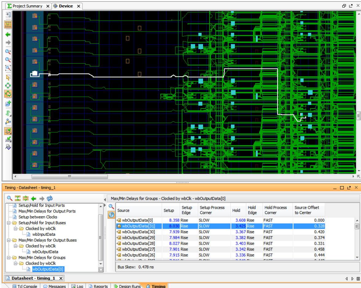
Figure 48: Detailed Routing View
