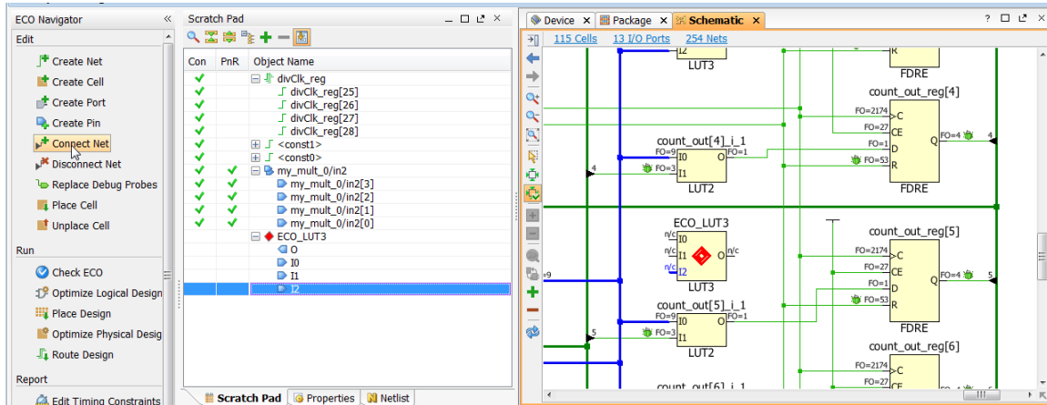
Figure 96: Scratch Pad and Schematic Showing ECO_LUT3 Added
