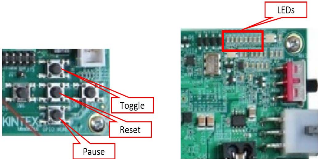
Figure 74: On-Board Push Buttons and LEDs
