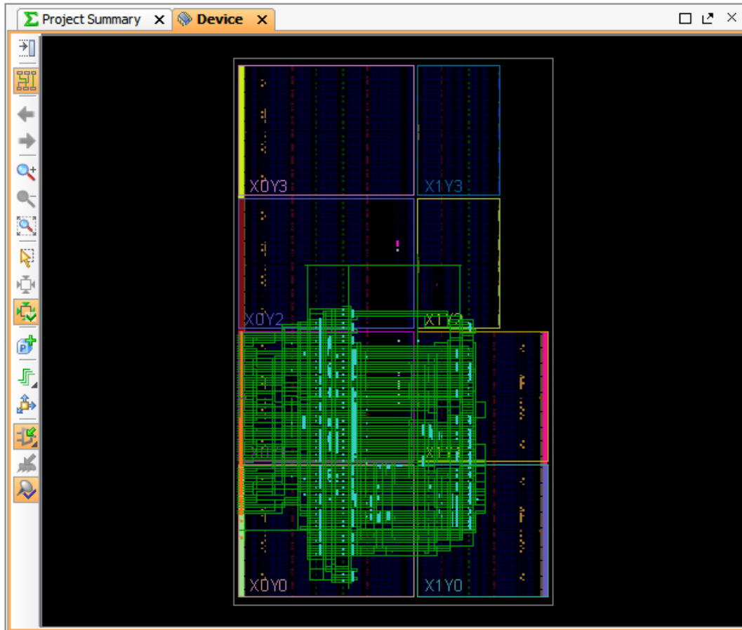
Figure 45: Device View
