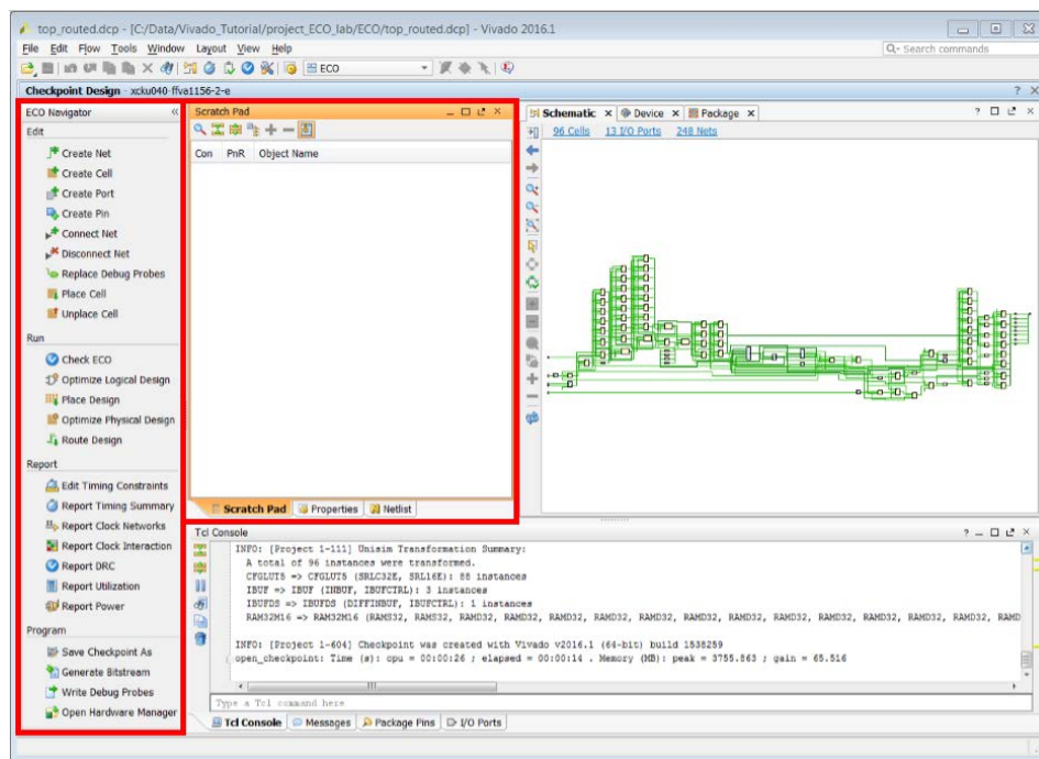
Figure 82: ECO Layout
