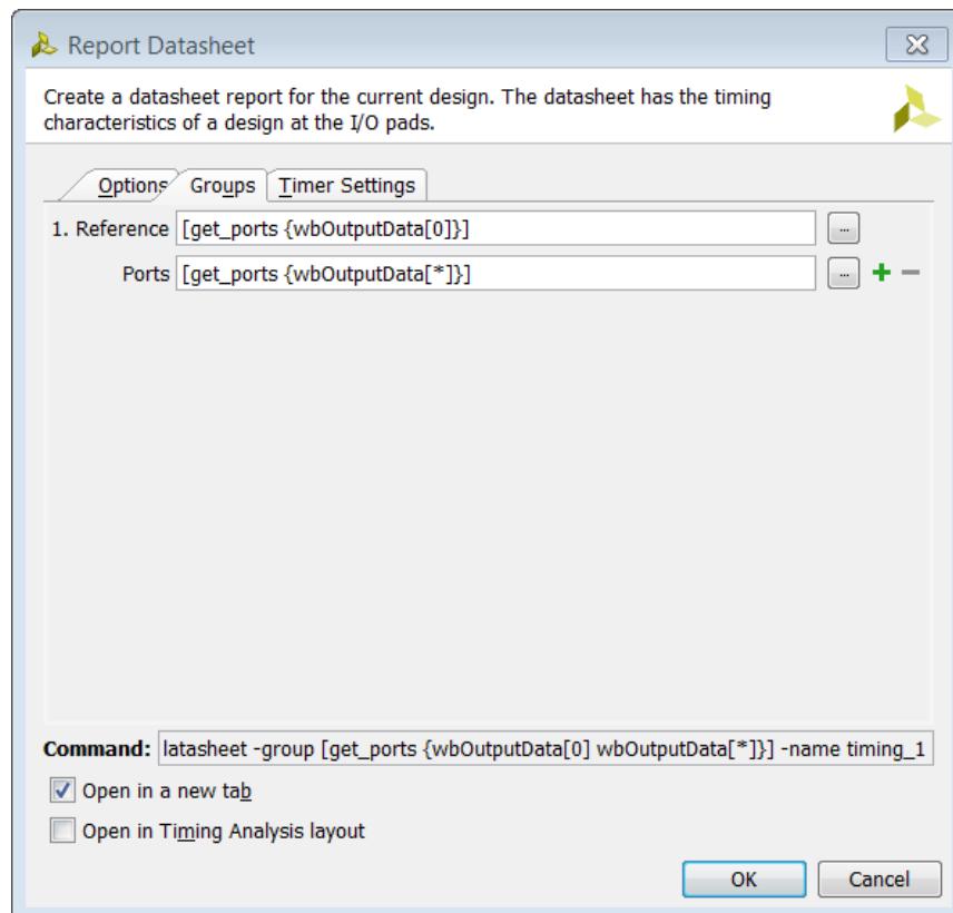
Figure 46: Report Datasheet
