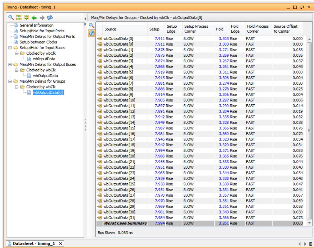
Figure 65: Report Datasheet – Final
