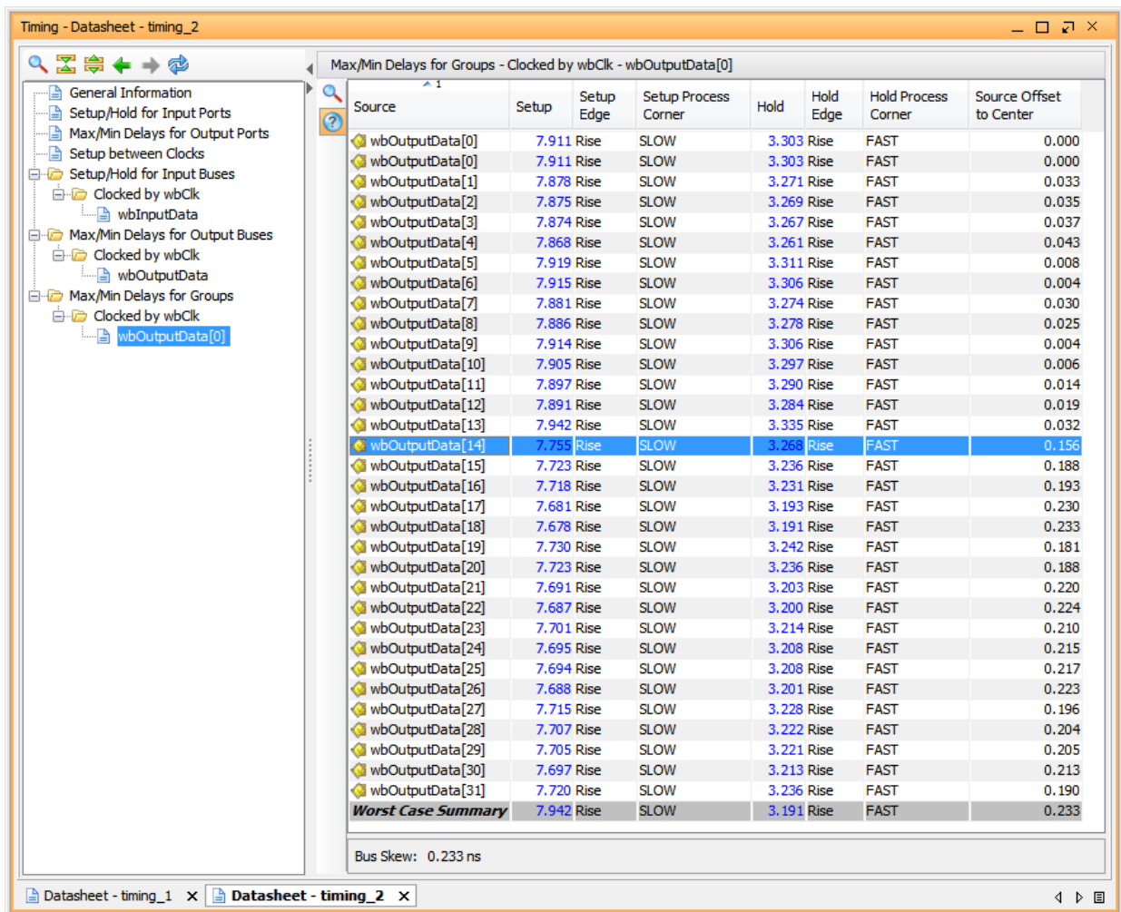
Figure 55: Report Datasheet – Improved Skew
