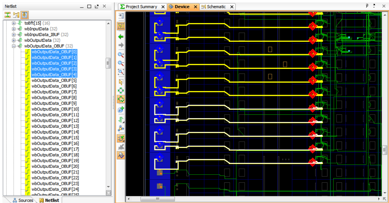
Figure 54: Improved Placement and Routing
