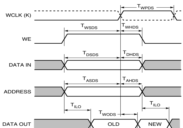
Dual Port RAM
