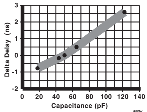
Figure 1: Delay Factor at Various Capacitive Loads
