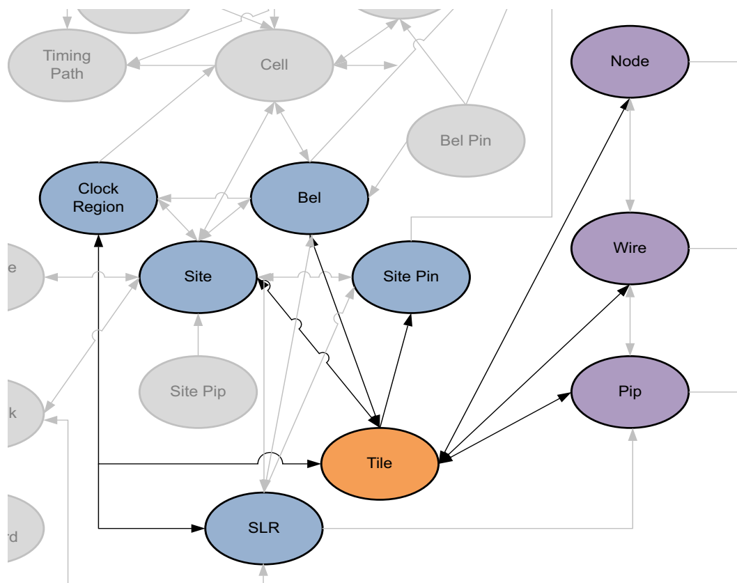
Figure 2-39: TILE Objects
