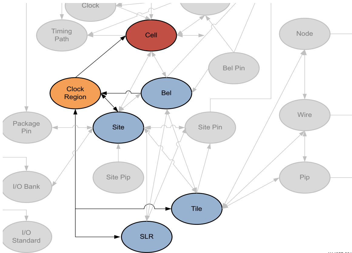
Figure 2-14: CLOCK_REGION Objects
