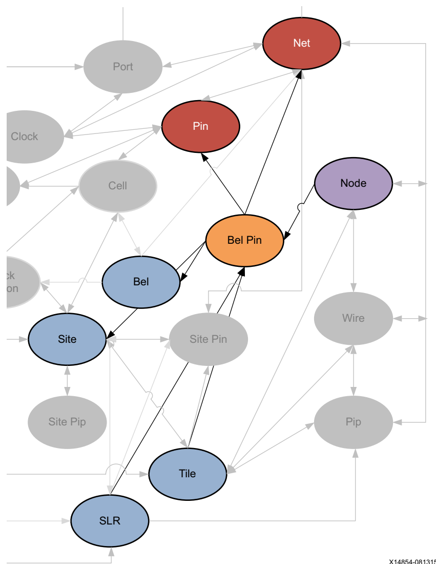
Figure 2-11: BEL_PIN Objects
