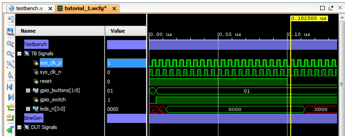
Figure 25: Viewing Reset and Clock Signals
