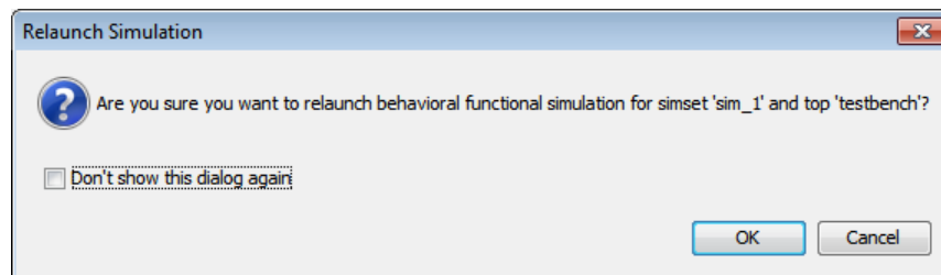
Figure 31: Confirm Relaunch
