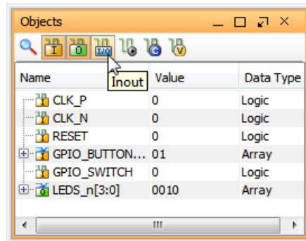
Figure 19: Object Filters
