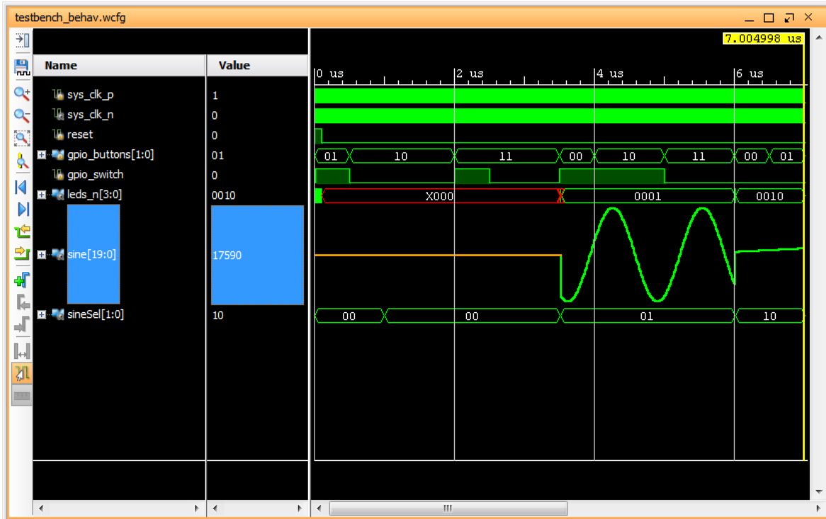
Figure 18: Design Bug - Wave View
