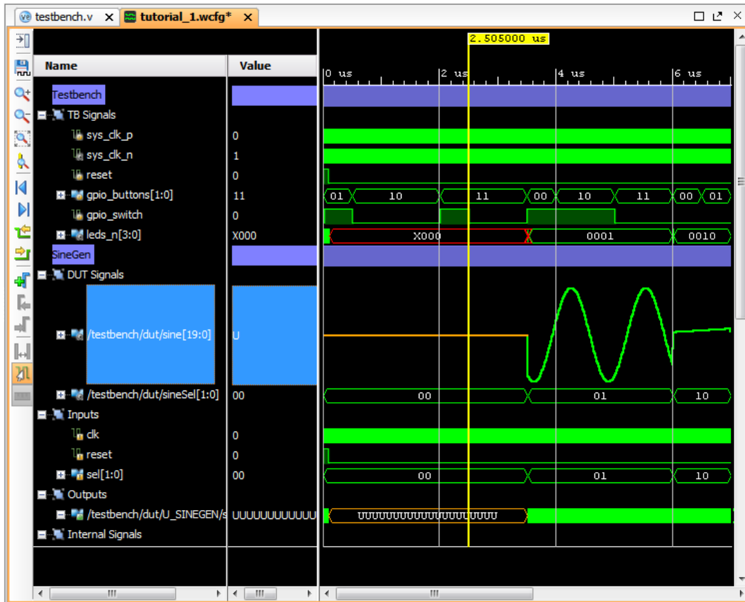
Figure 23: Simulation Waveform at Time 705 ns
