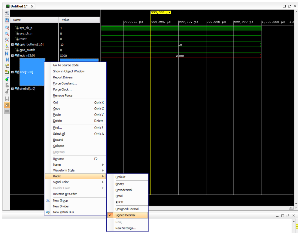
Figure 17: Enable Radix
