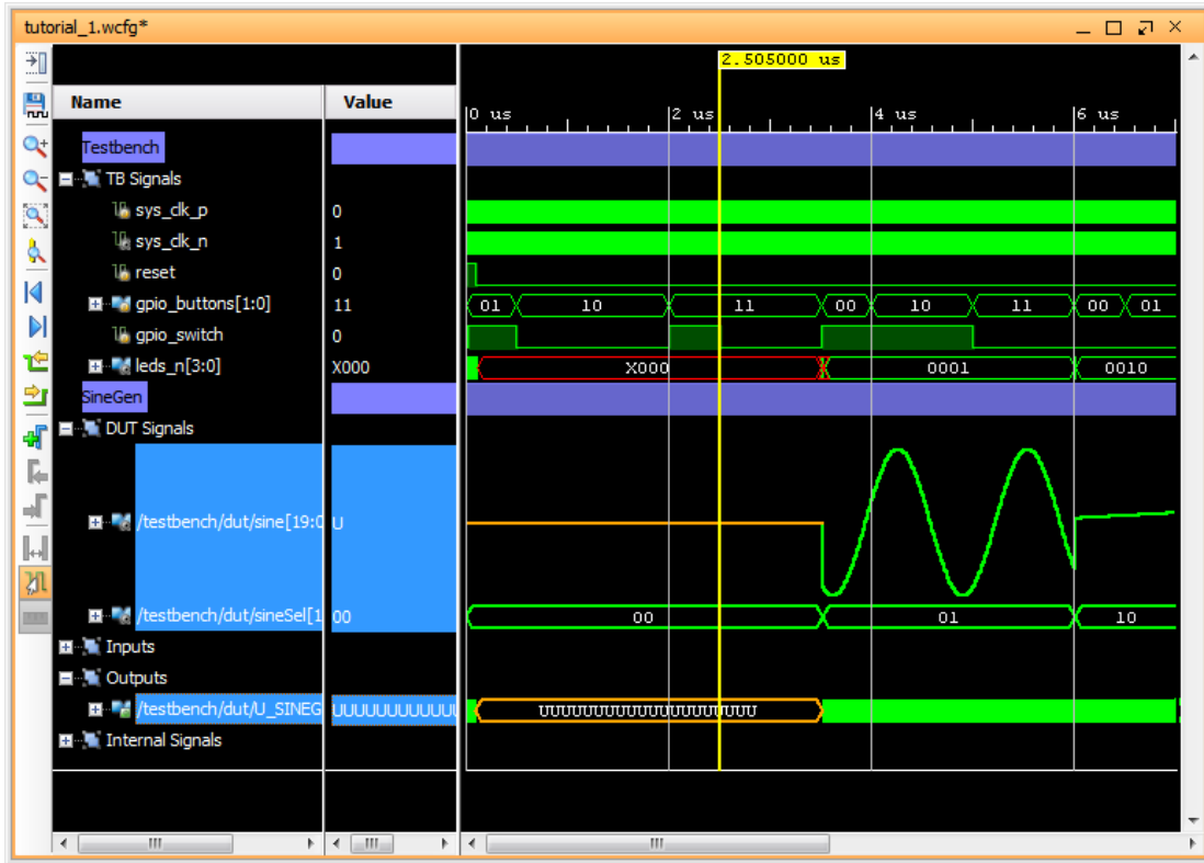
Figure 21: Long Signal Names
