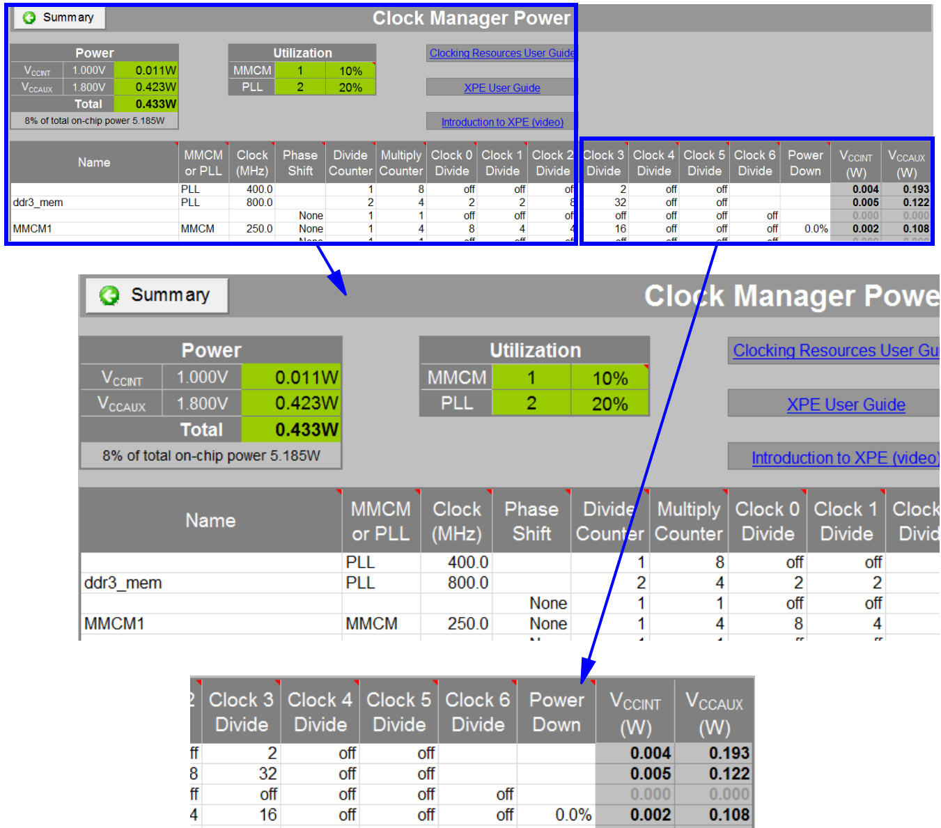
Figure 26: Clock Manager Power Sheet (7 Series)
