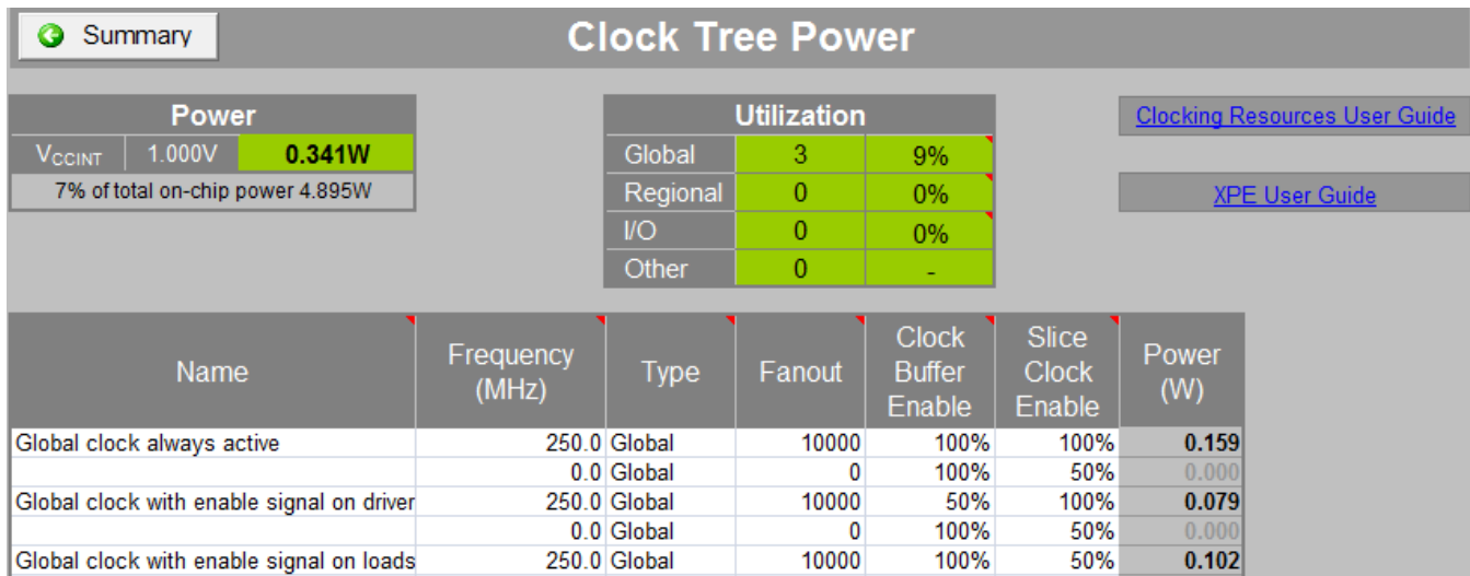
Figure 20: Clock Tree Power Sheet (7 Series)
