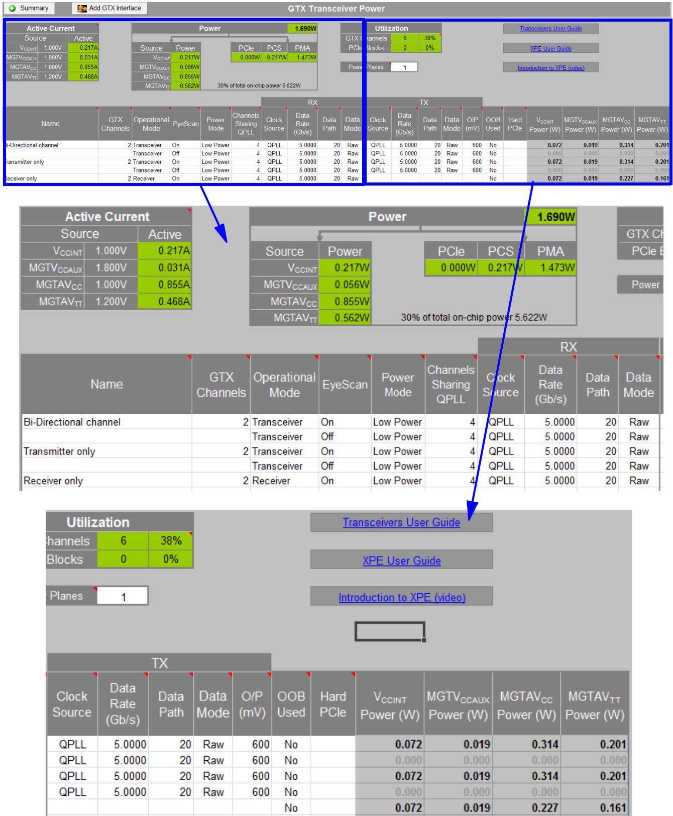
Figure 28: GT Power Sheet (Kintex-7) Illustrating Data Rate and Power Estimates
