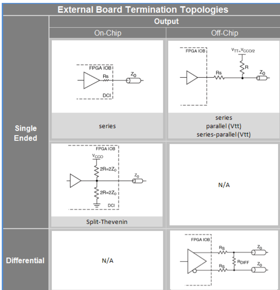
Figure 24: External I/O Termination Topologies (Virtex-6 and 7 Series)
