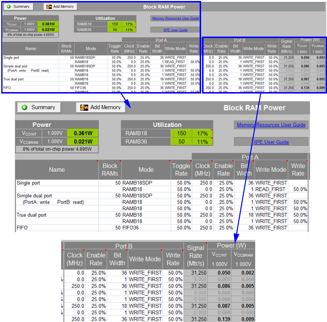
Figure 25: Block RAM Sheet - Effect of Block RAM Configuration Modes and Bit Widths on Power Estimates (7 Series)
