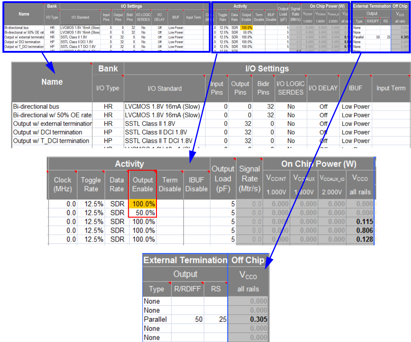
Figure 23: I/O Sheet - Effect of Output Enable Rate on Power Estimates for Inputs, Outputs, and Bidirectional I/Os (7 Series)
