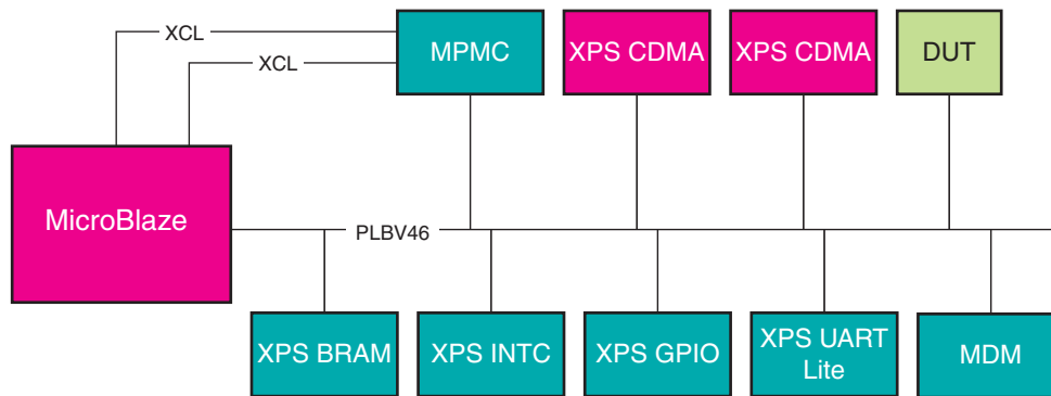
Figure 17: Virtex-6 FPGA System with the XPS USB2 Device as the DUT
