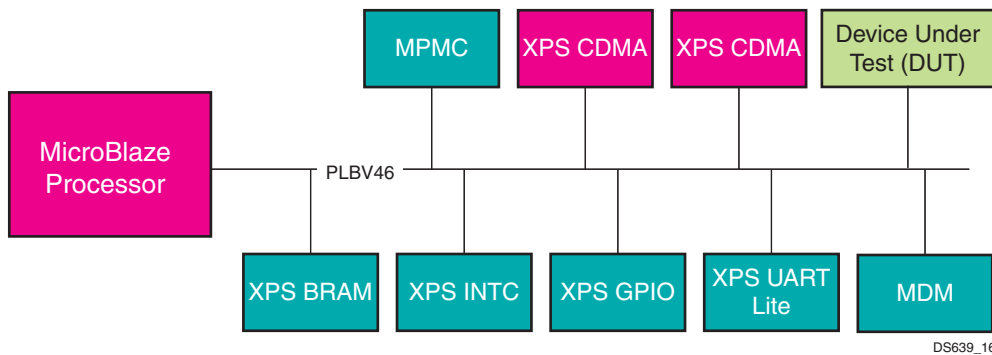
Figure 16: Spartan-3A FPGA System with the XPS USB2 Device as the DUT
