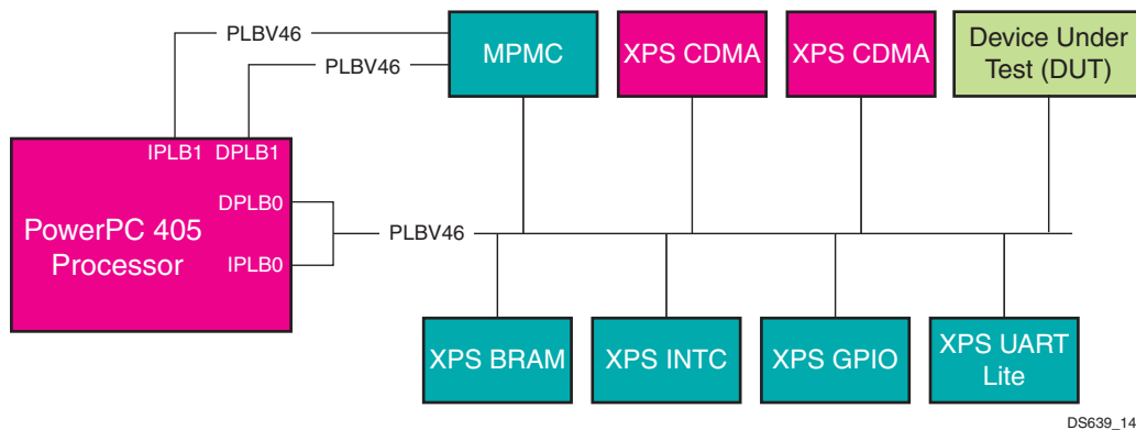
Figure 14: Virtex-4 FX FPGA System with the XPS USB2 Device as the DUT
