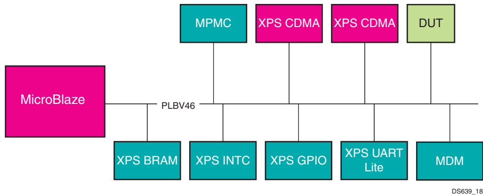
Figure 18: Spartan-6 FPGA System with the XPS USB2 Device as the DUT
