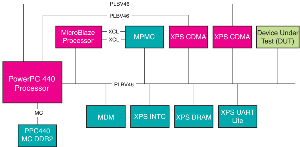
Figure 15: Virtex-5 LX FPGA System with the XPS USB2 Device as the DUT
