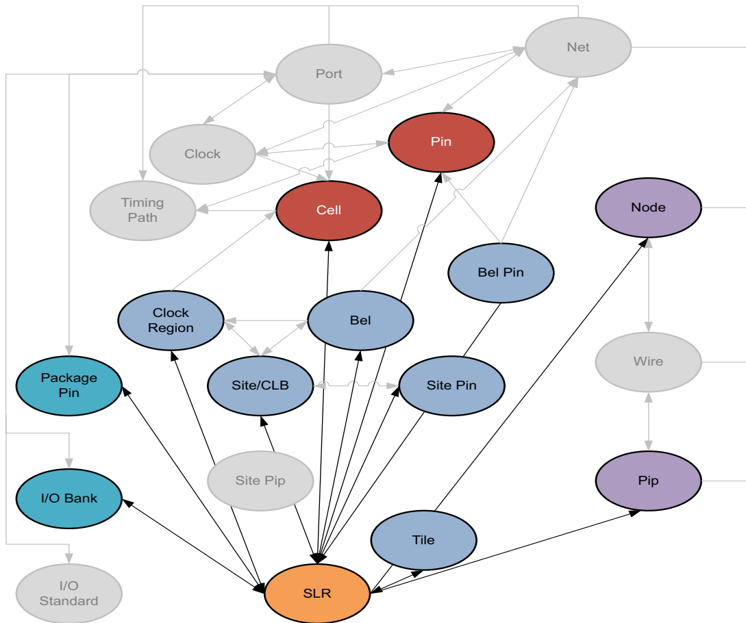
Figure 2-38: SLR Objects
