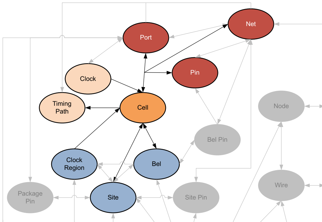
Figure 2-12: CELL Objects
