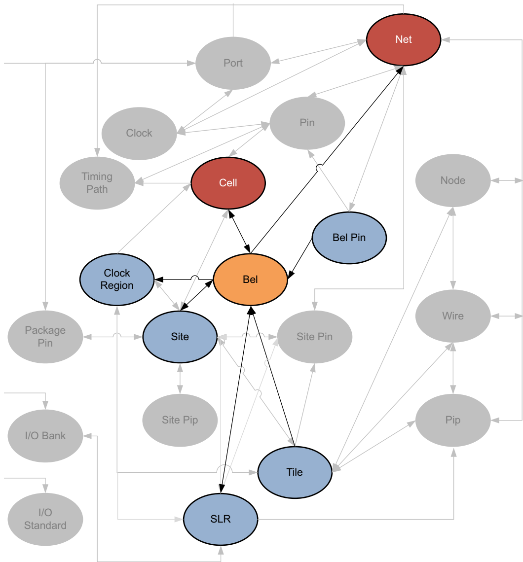
Figure 2-10: BEL Objects
