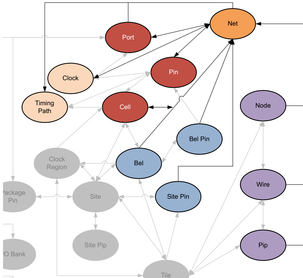
Figure 2-29: NET Objects
