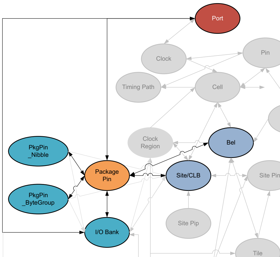
Figure 2-31: PACKAGE_PIN Objects
