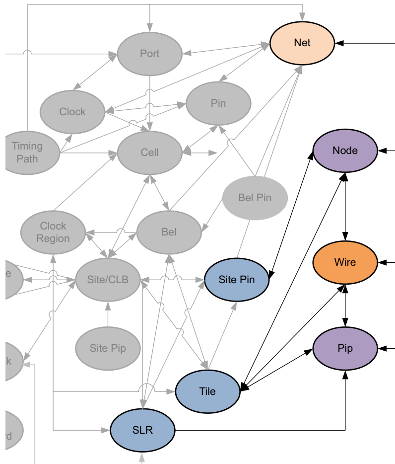
Figure 2-41: WIRE Objects
