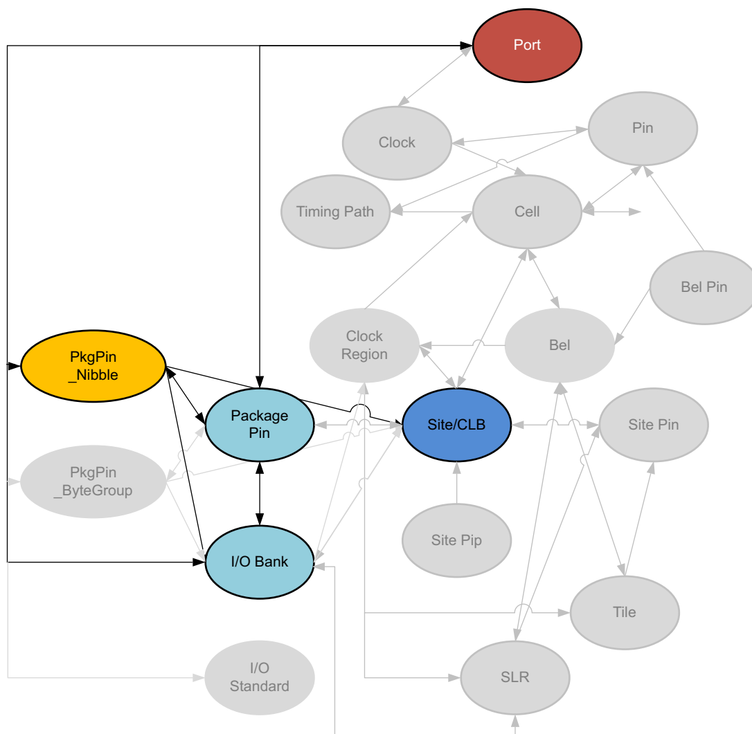
Figure 2-35: PKGPIN_NIBBLE Objects
