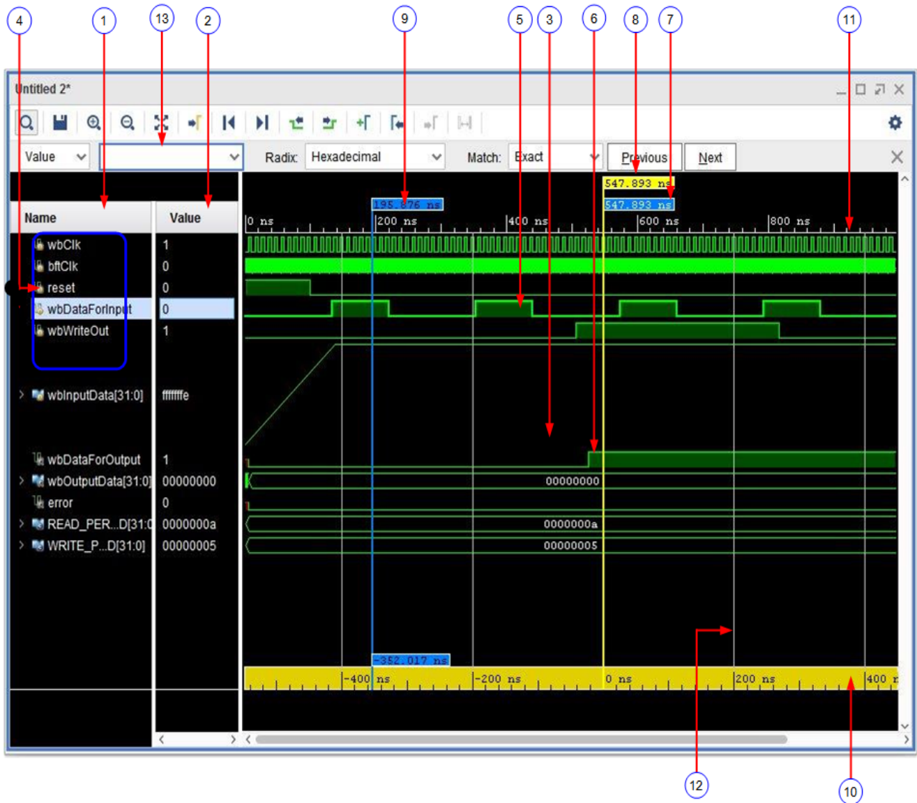
Figure 4-11: Wave Window
