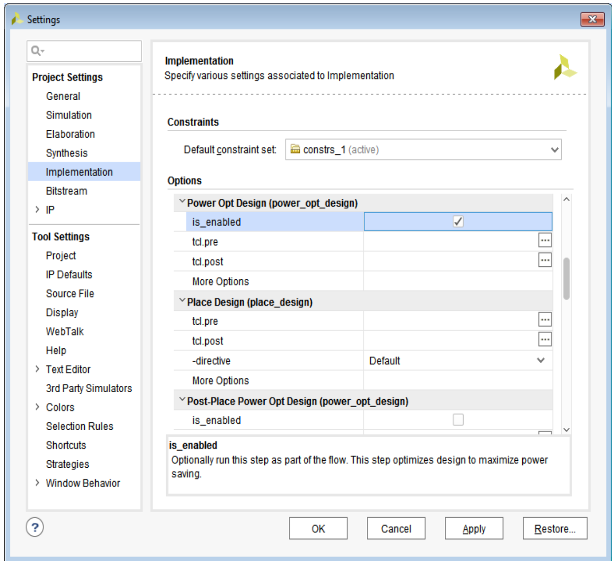
Figure 4-12: Power Optimization Option
