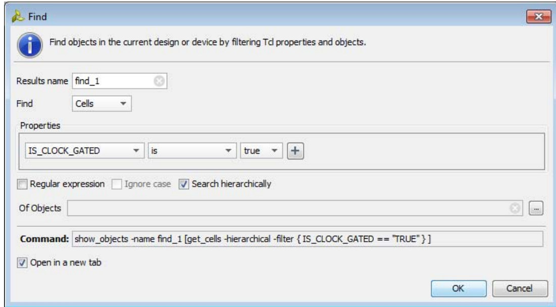
Figure 4-15: Finding Power Optimized Cells
