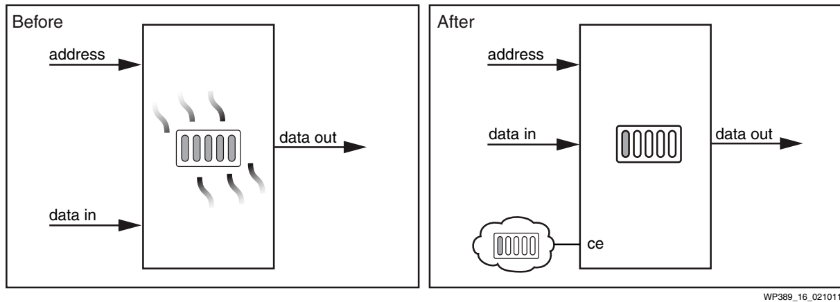
Figure 4-10: Clock Gating Optimizations Using Block RAM Enables
