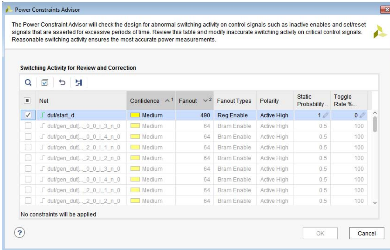
Figure 4-6: Power Constraints Advisor
