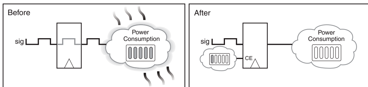
Figure 4-9: Intelligent Clock Gating
