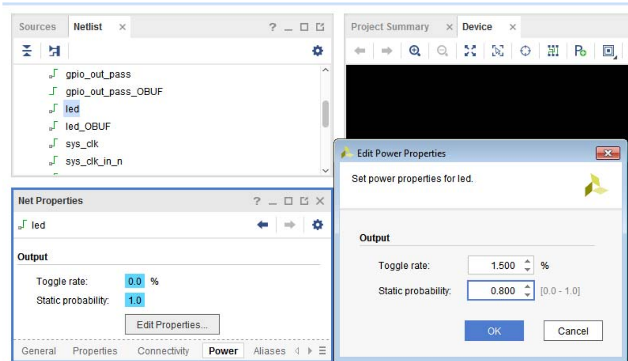
Figure 4-5: Power View in Net Properties
