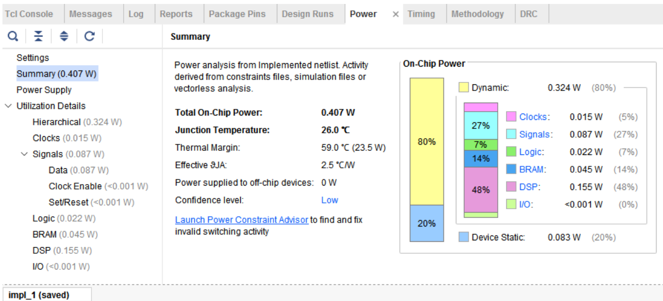
Figure 1-4: Vivado Power Analysis
