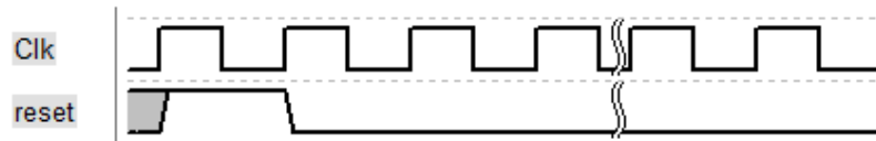
Figure 5-7: Reset Signal Duration
