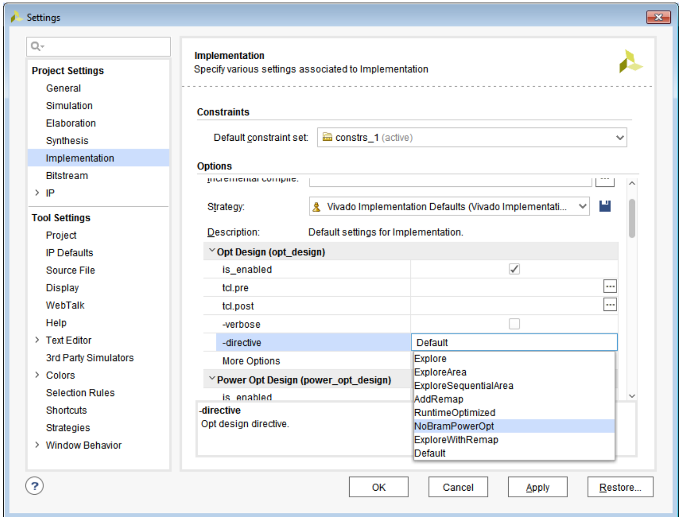
Figure 4-11: Disabling BRAM Power Optimization During Opt Design
